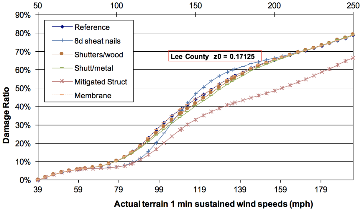
Figure 73. Mitigation measures for frame homes.
