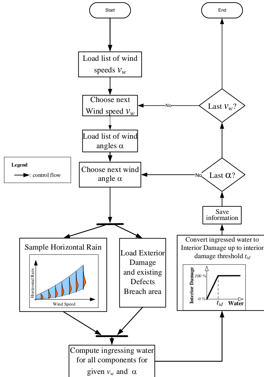
Figure 57. Flowchart of the interior damage model
