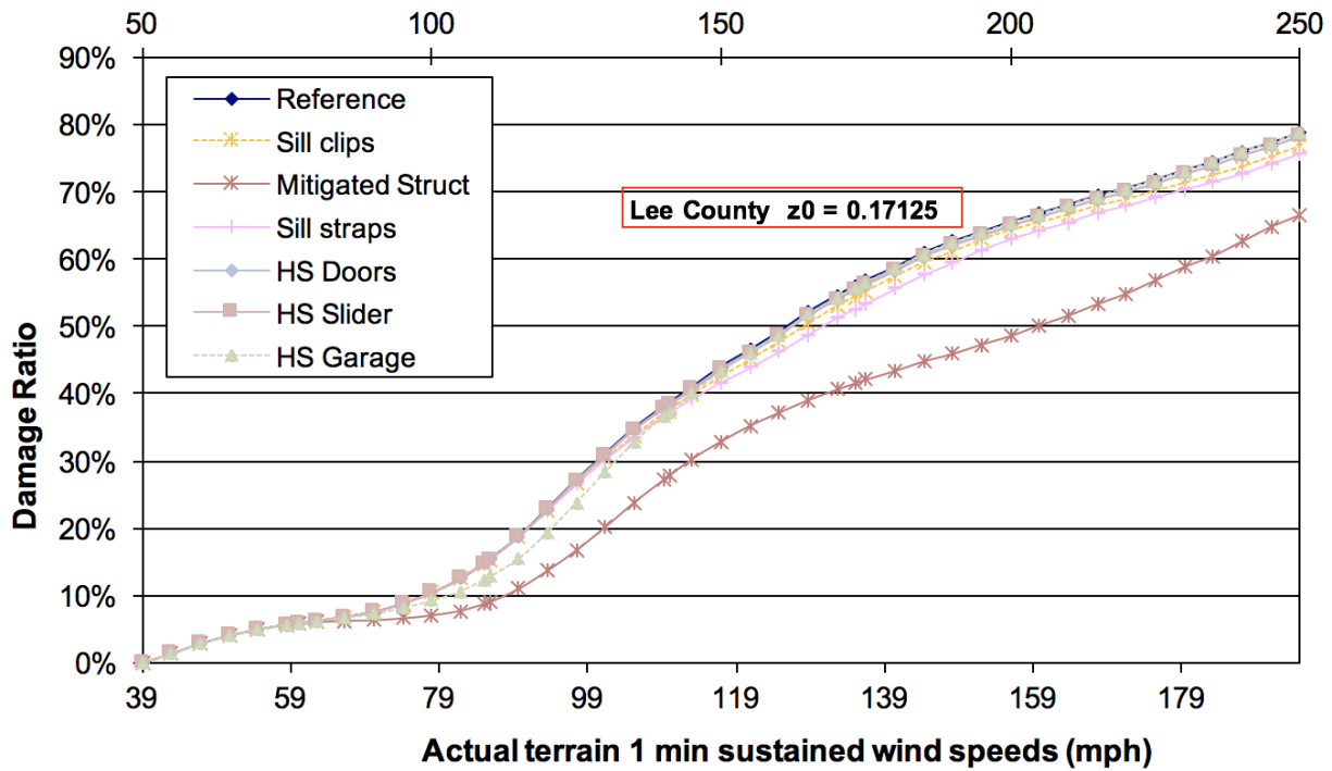
Figure 74. Mitigation measures for frame homes.
