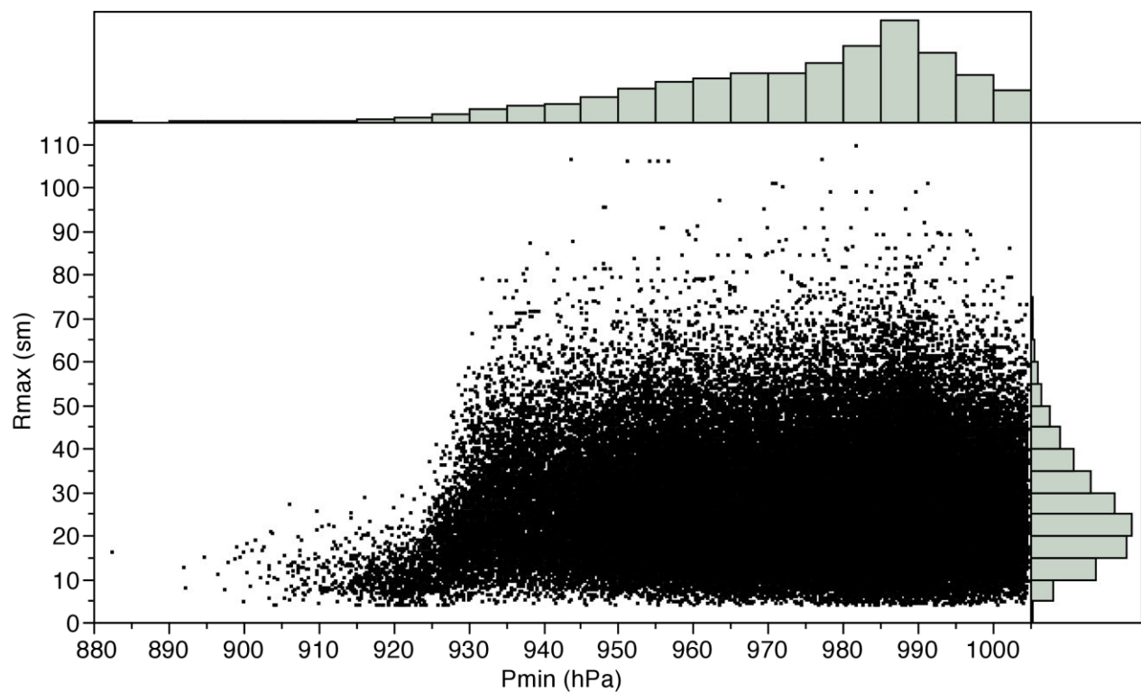
Figure 37. Representative scatter plot of the model input radius of maximum wind (y axis) versus minimum sea-level air pressure at landfall (mb). Relative histograms for each quantity are also shown.
