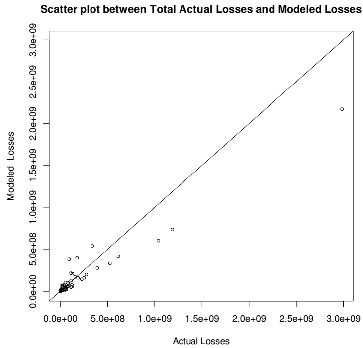
Figure 46. Scatter plot between total actual vs. total modeled losses (Personal Residential).
