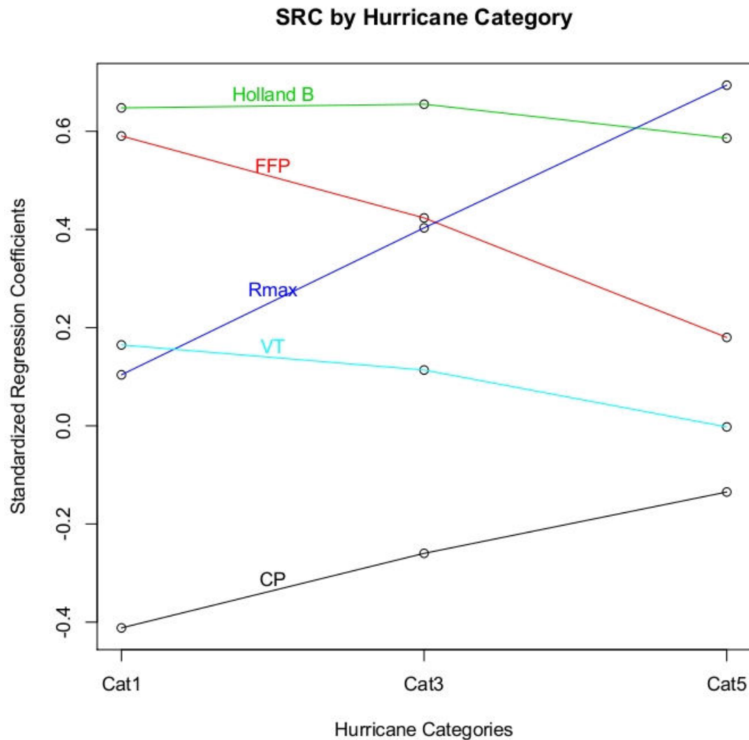
Figure 44. SRCs for Expected Loss Cost for all Input Variables for all Hurricane Categories.
