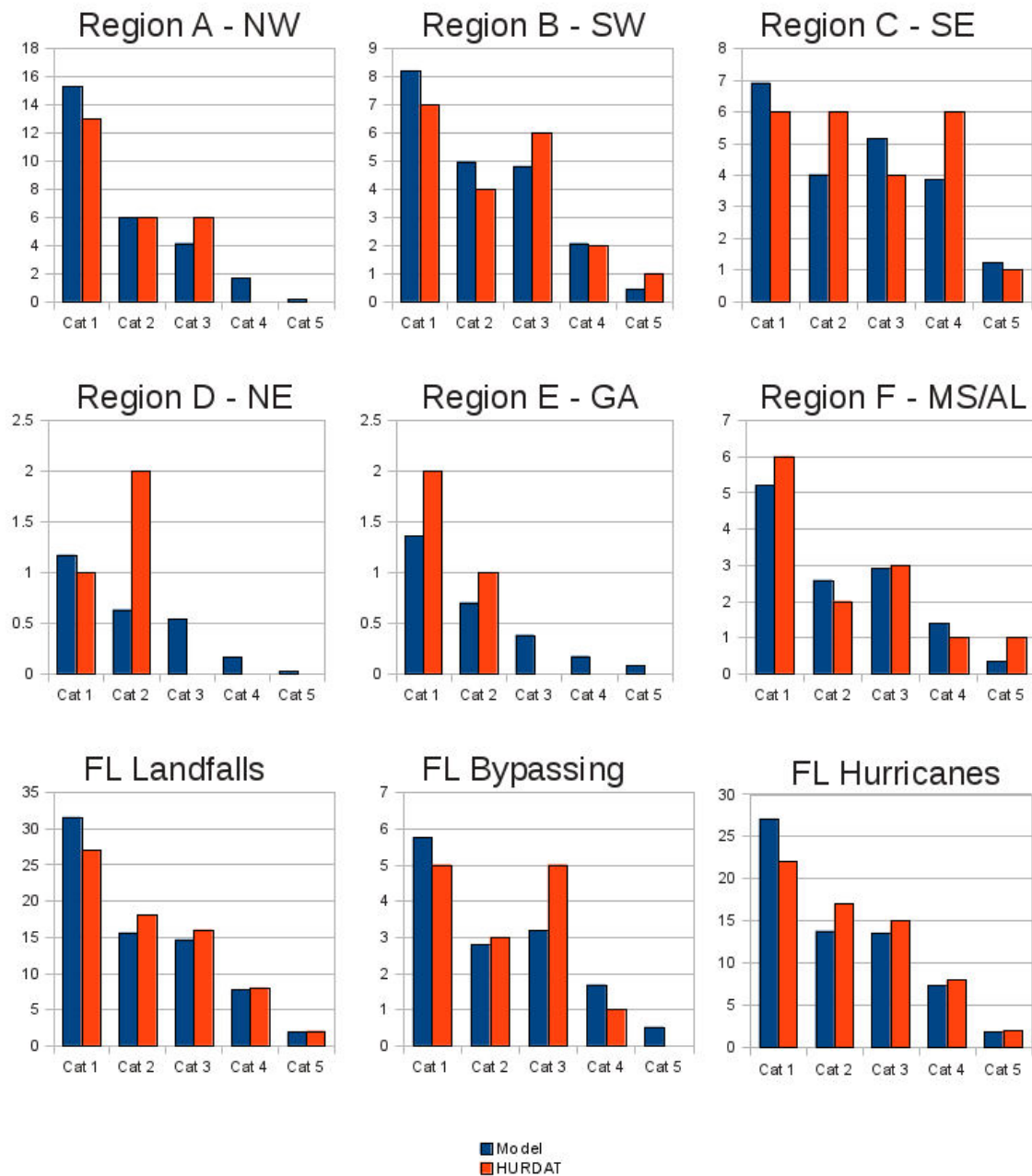
Figure 32. Form M-1 comparison of modeled and historical landfalling hurricane frequency (storms occurring in 114 years) for Regions A–F, FL statewide landfalls (one per FL region), FL bypassing storms, and FL state-wide hurricanes.
