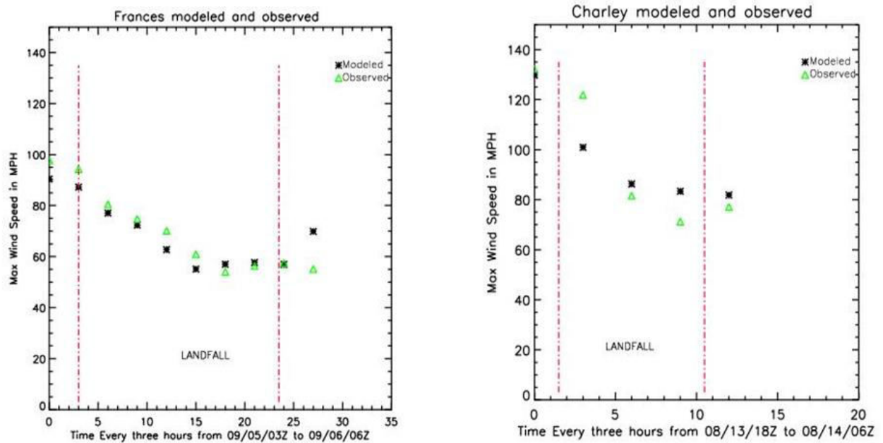
Figure 30. Observed (green) and modeled (black) maximum sustained surface winds as a function of time for 2004 Hurricanes Frances (left) and Charley (right). Landfall is represented by the vertical dash-dot red line at the left and time of exit as the red line on the right.
