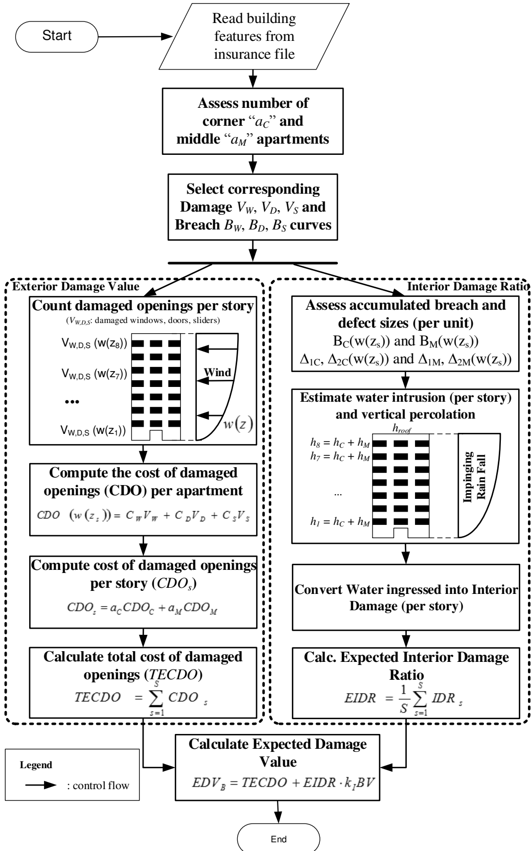
Figure 62. Exterior and interior damage assessment for MHB.
