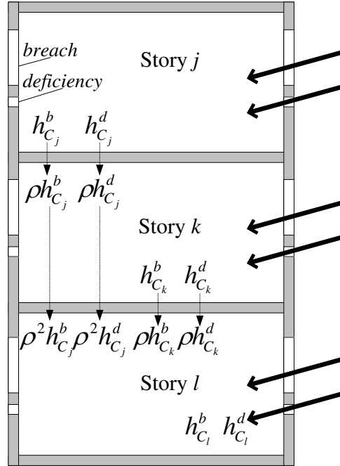
Figure 68. Diagram of water intrusion through breaches, deficiencies and percolation in a 3-story building.
