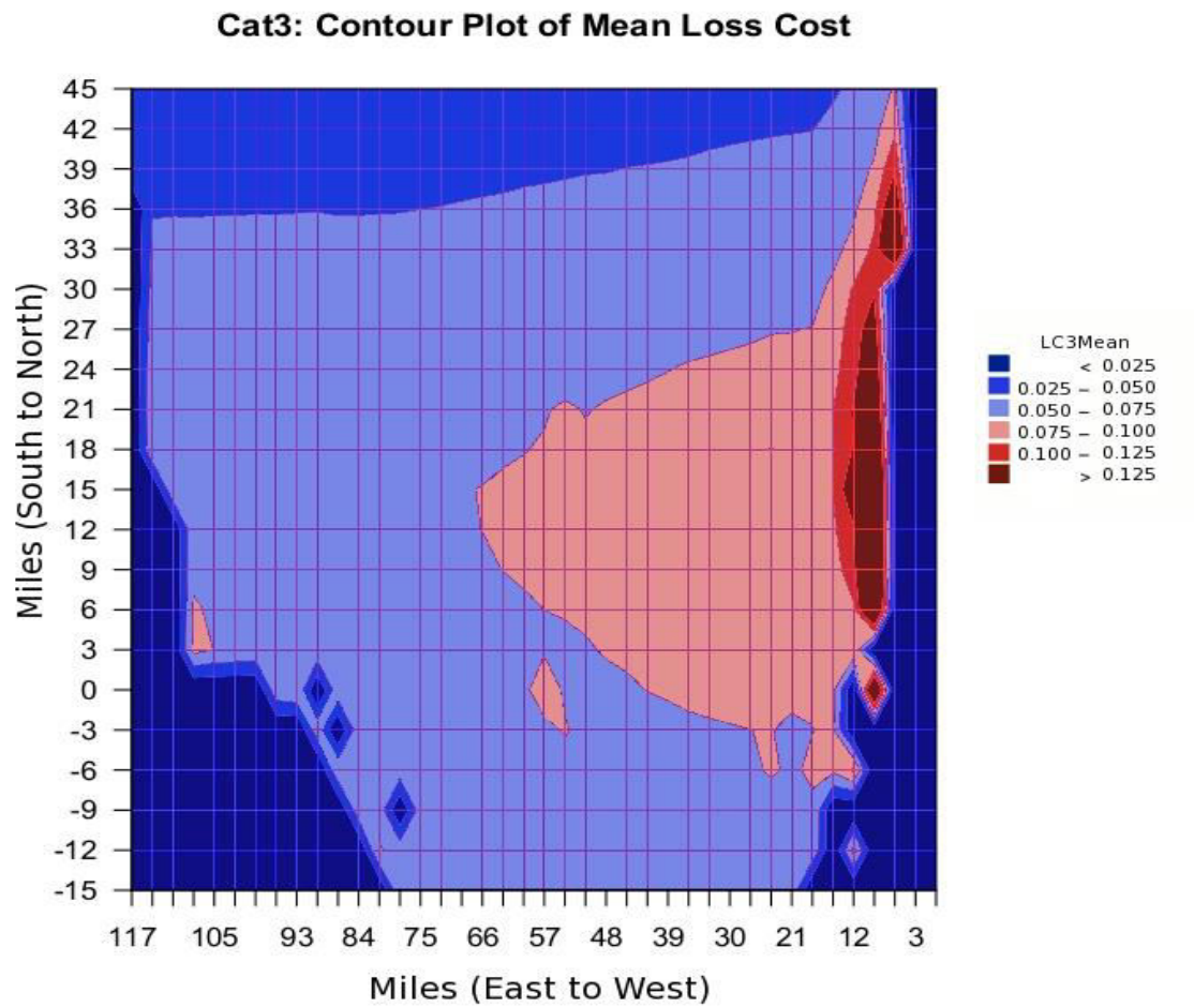
Figure 56. Contour Plot of Loss Cost for a Category 3 Hurricane.
