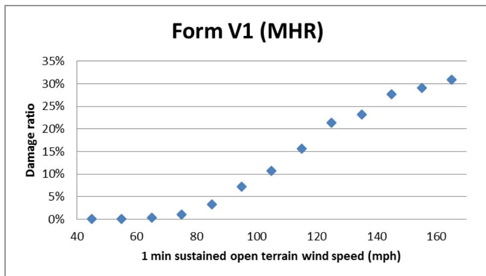
Figure 79. Structure damage vs. 1 minute sustained wind speed.
