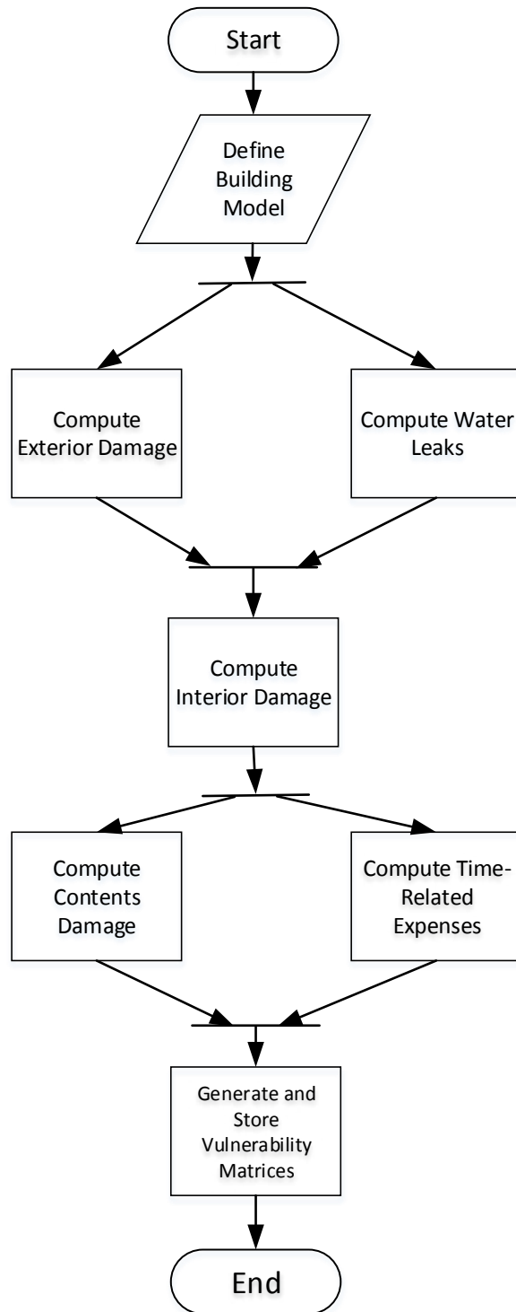
Figure 69. Derivation of contents and additional living expenses vulnerabilities for PR.
