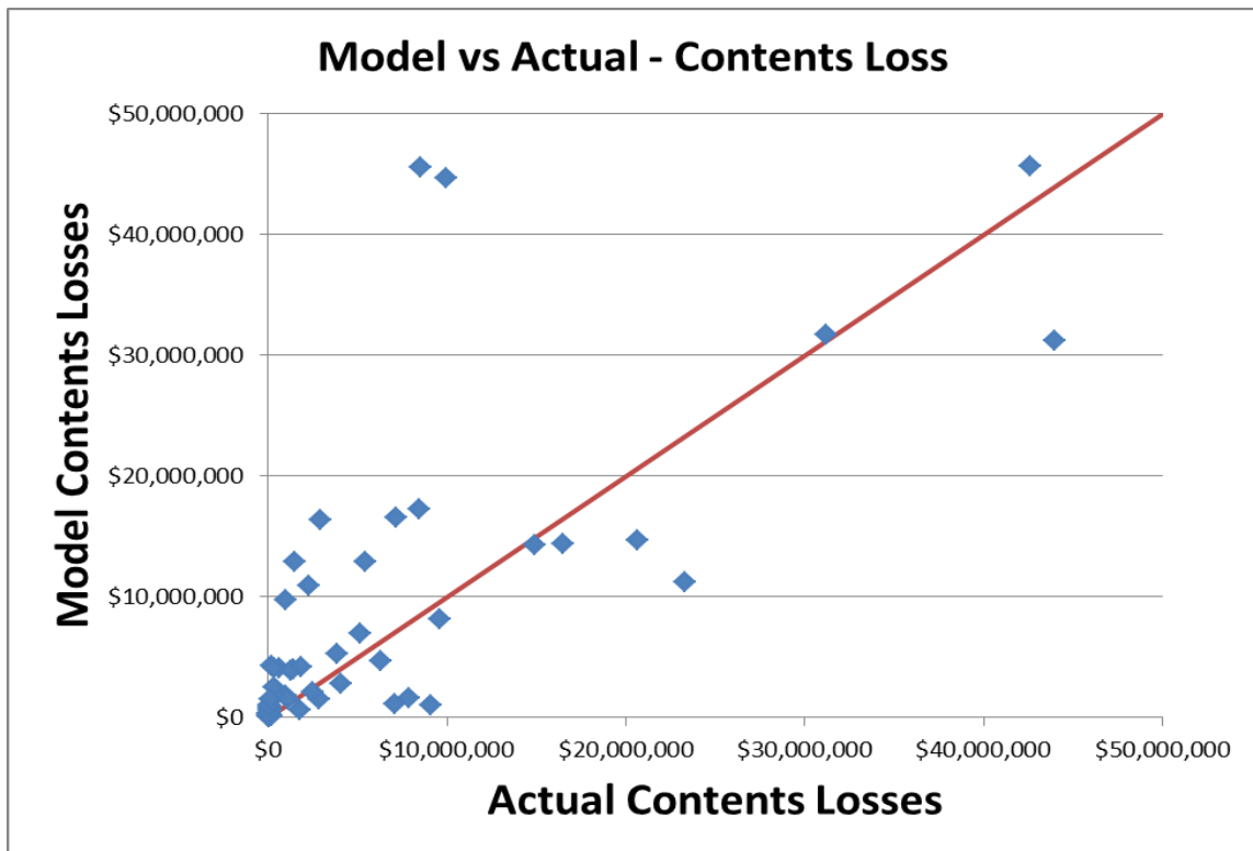
Figure 72. Model vs. Actual-Contents Loss.
