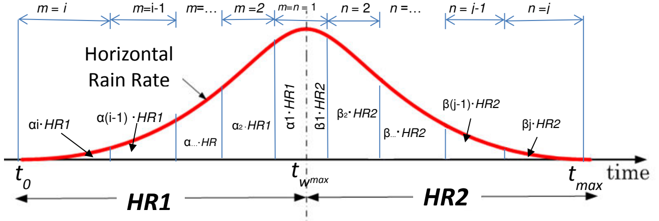
Figure 67. Horizontal rain rate as a function of storm duration.
