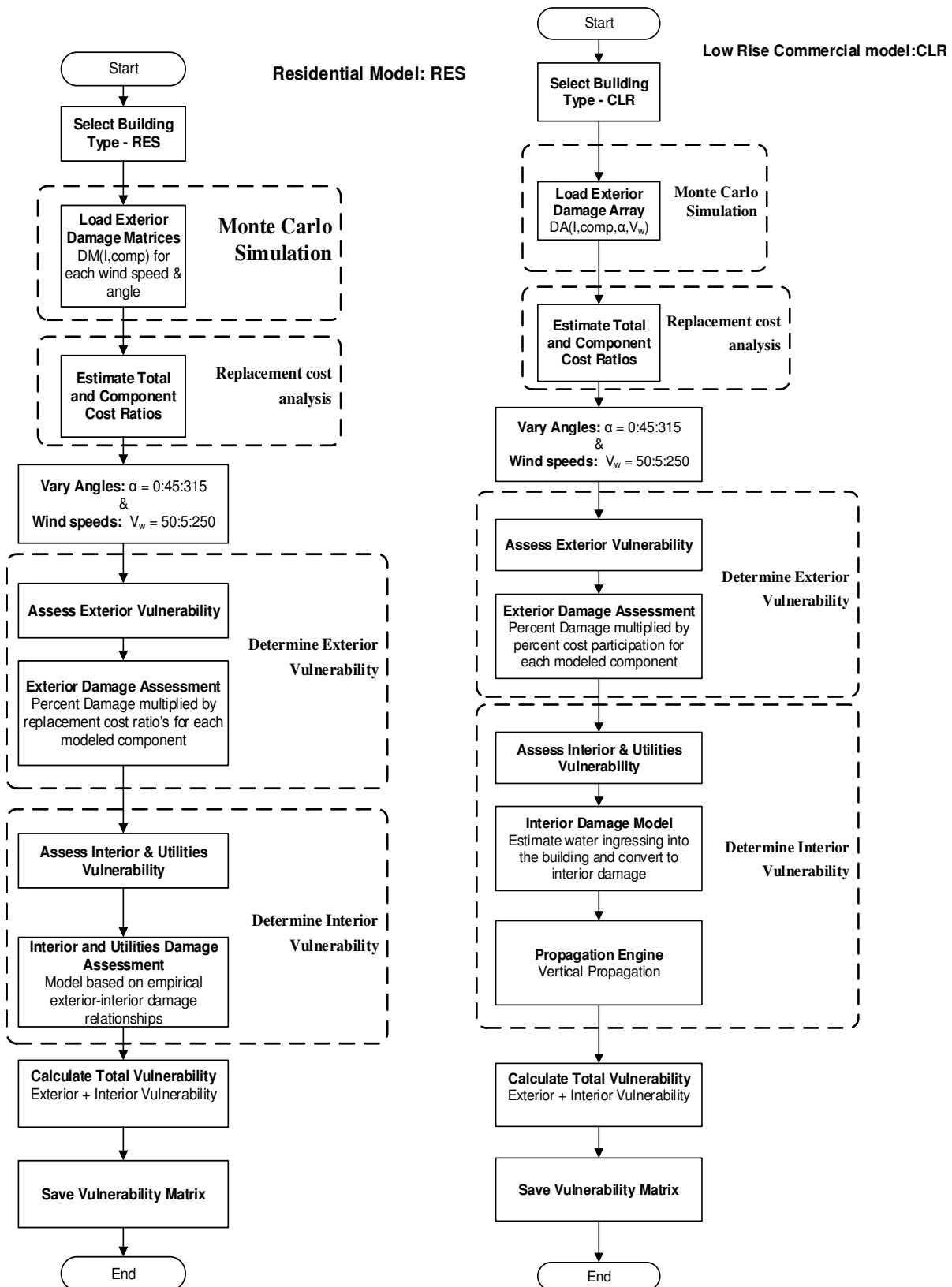
Figure 61. Procedure to create vulnerability matrix.
