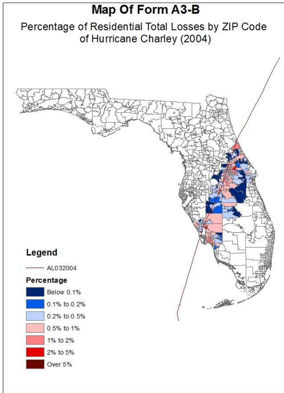
Figure 93. Percentage of residential total losses by ZIP code of Hurricane Charley (2004).
