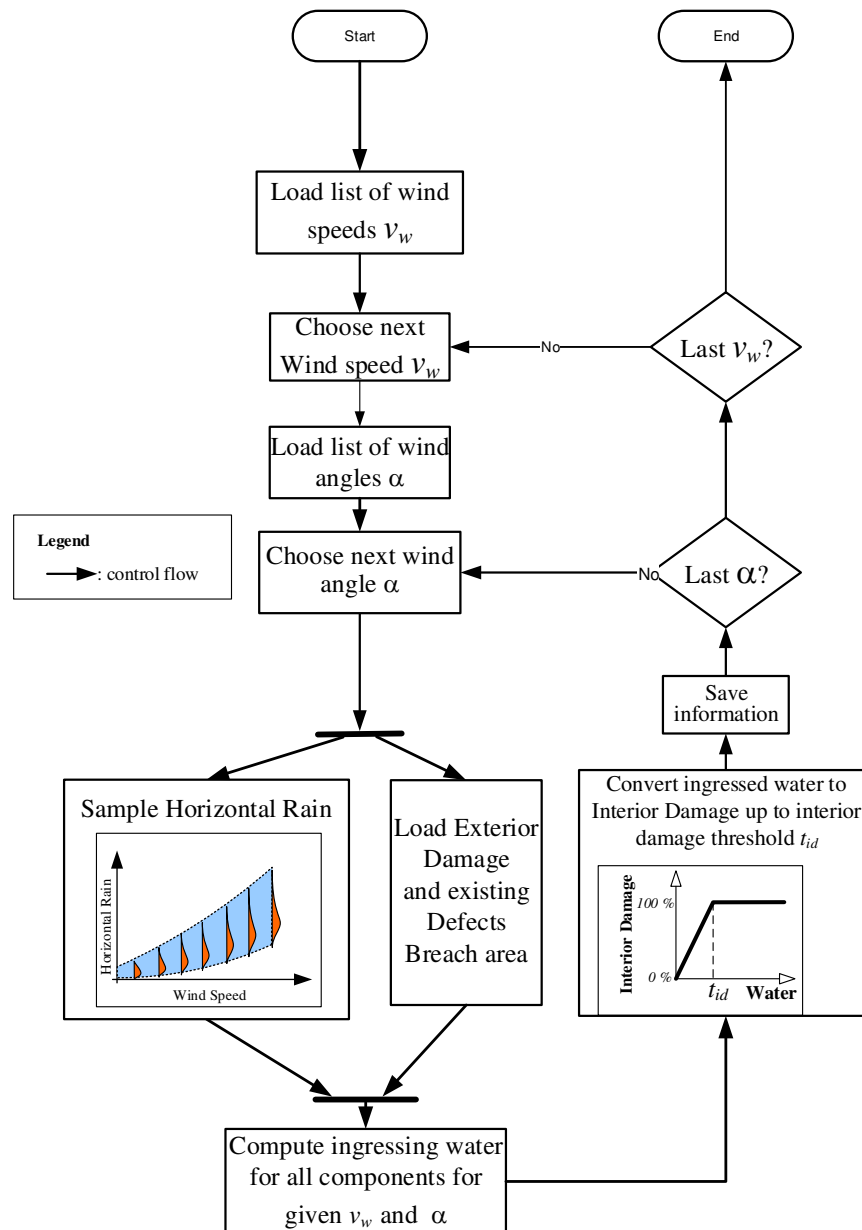
Figure 66. Flowchart of the interior damage model.
