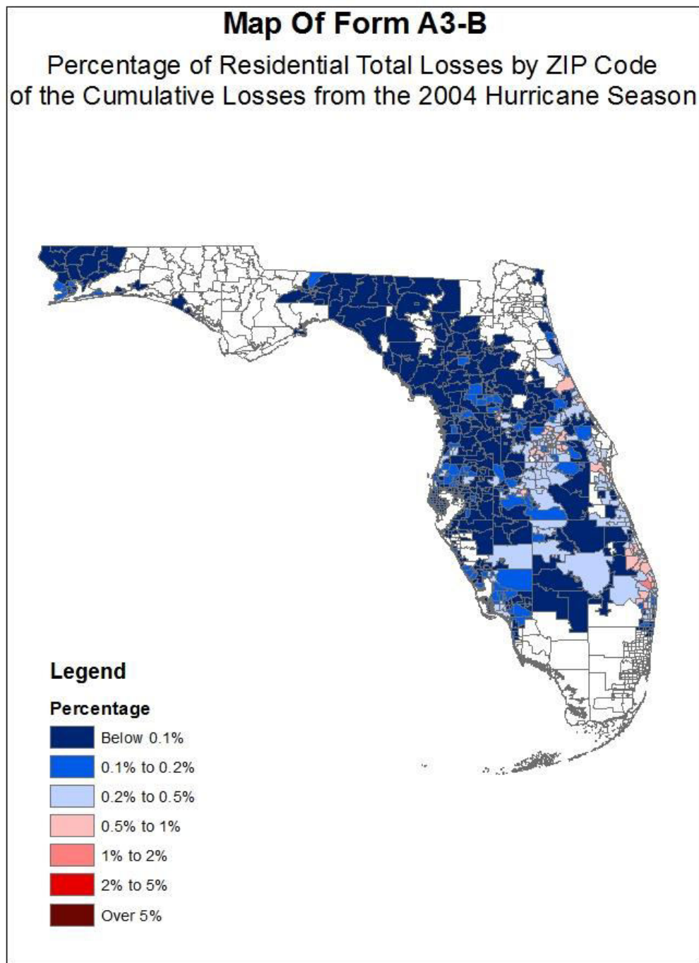
Figure 97. Percentage of residential total losses by ZIP code of the cumulative losses from the 2004 Hurricane Season.
