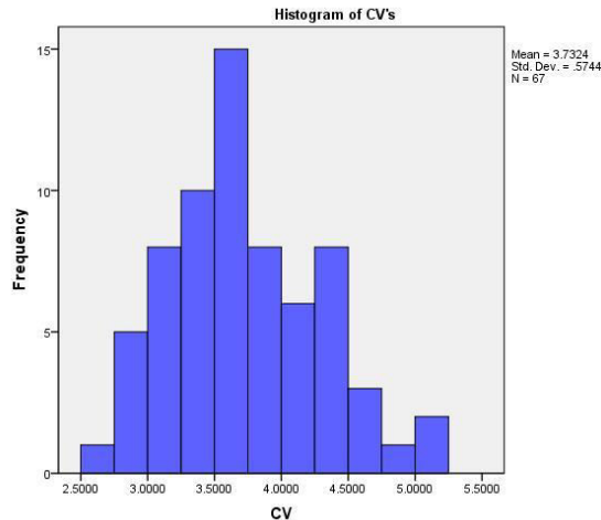
Figure 43. Histogram of CVs for all counties combined.
