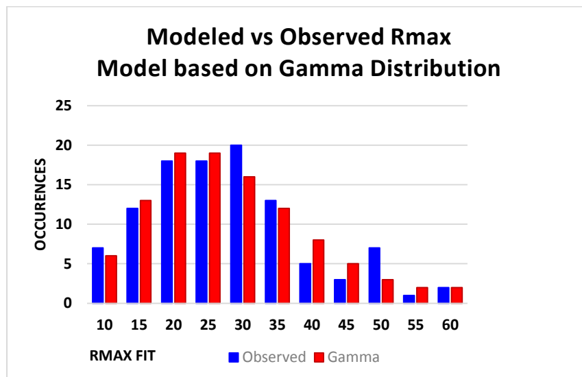
Figure 41. Observed and expected distribution using a gamma distribution.
