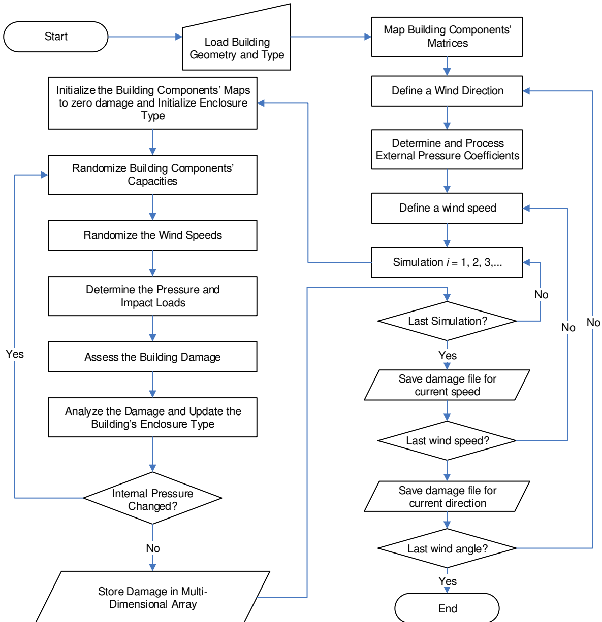
Figure 60. Monte Carlo simulation procedure to predict damage.
