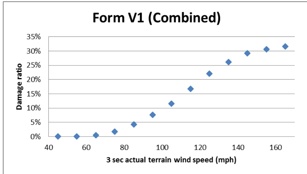
Figure 70. Structure damage vs. 3 sec actual terrain wind speed.
