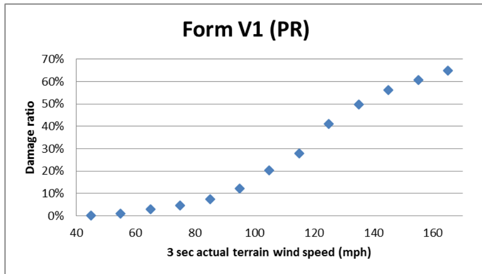
Figure 72. Structure damage vs. 3 sec actual terrain wind speed.
