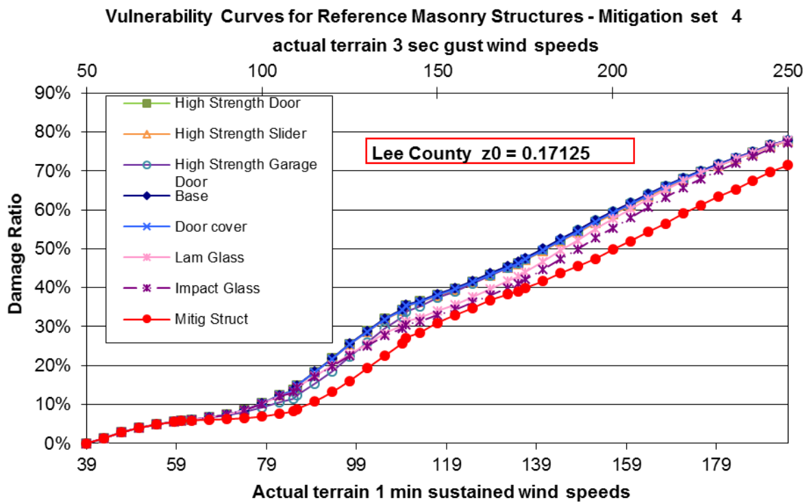
Figure 77. Mitigation measures for masonry homes.
