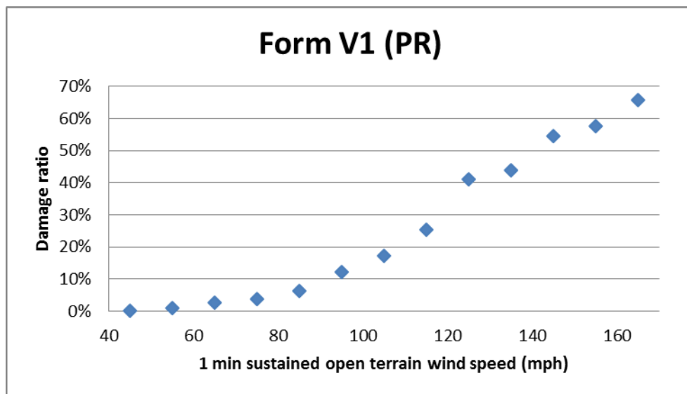
Figure 73. Structure damage vs. 1 minute sustained wind speed.
