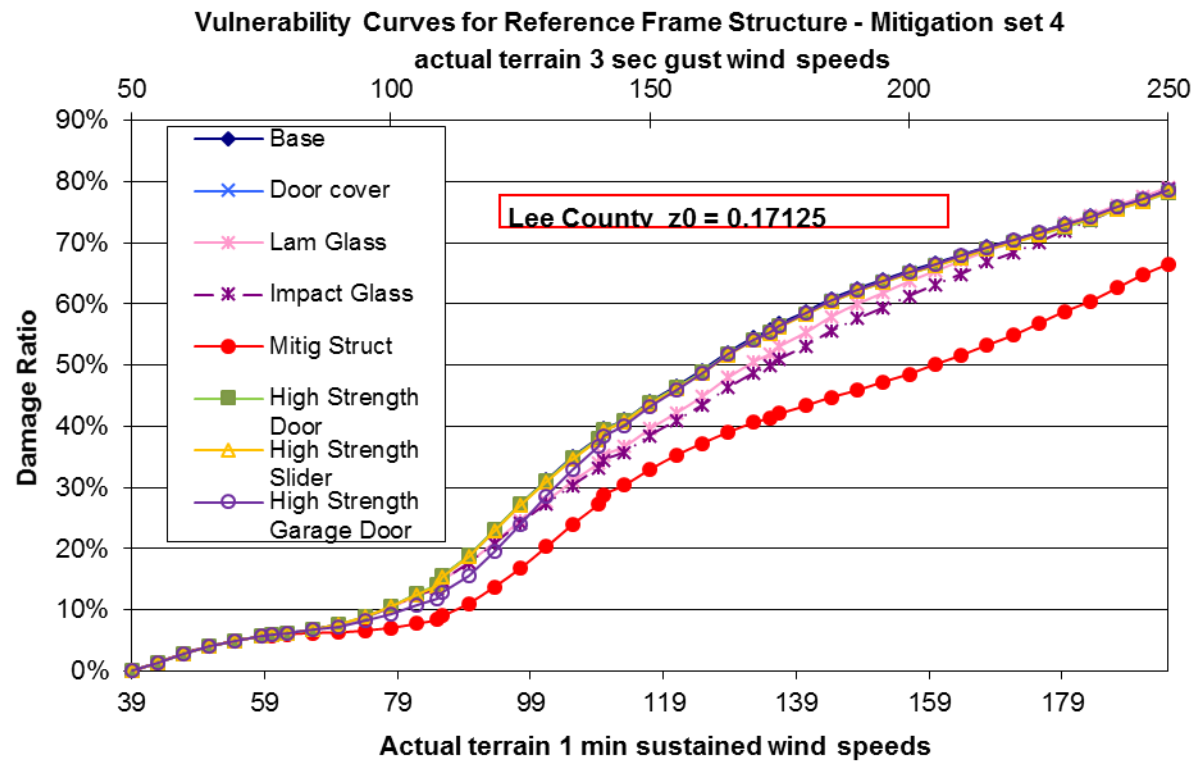
Figure 79. Mitigation measures for frame homes.
