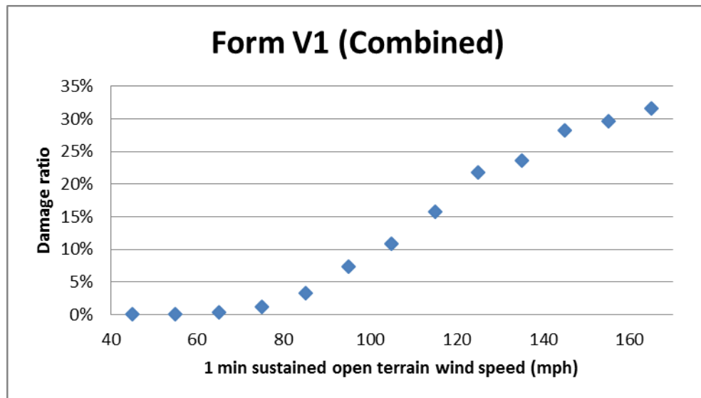
Figure 71. Structure damage vs. 1 minute sustained wind speed.
