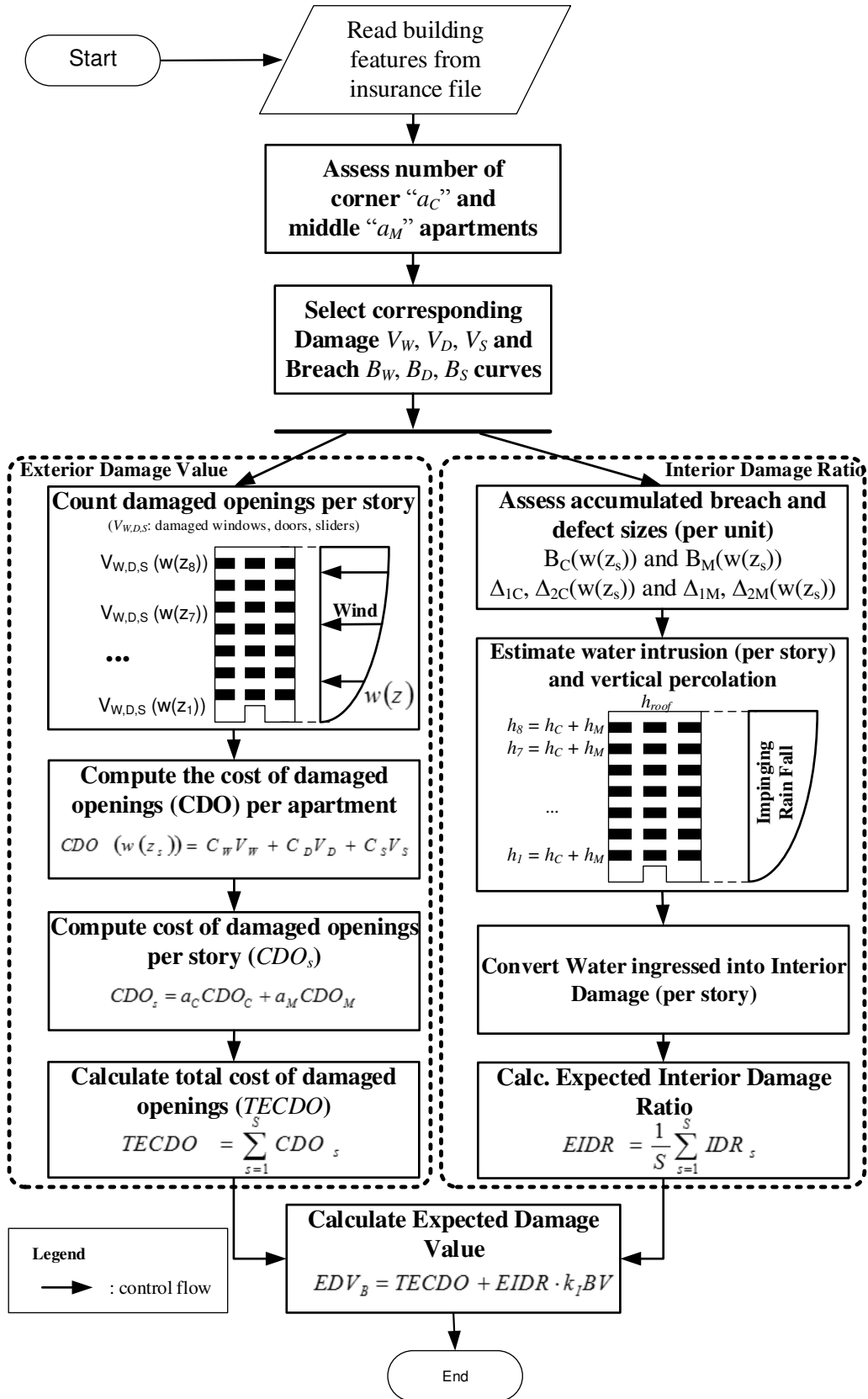
Figure 59. Exterior and interior damage assessment for MHB.
