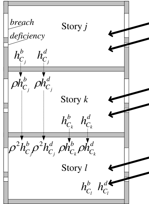
Figure 65. Diagram of water intrusion through breaches, deficiencies and percolation in a 3-story building.
