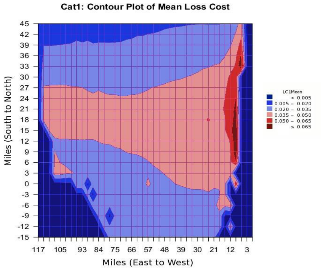
Figure 52. Contour Plot of Loss Cost for a Category 1 Hurricane.
