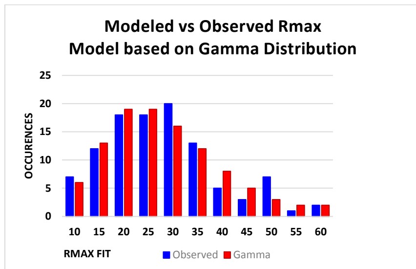
Figure 38. Observed and expected distribution using a gamma distribution.
