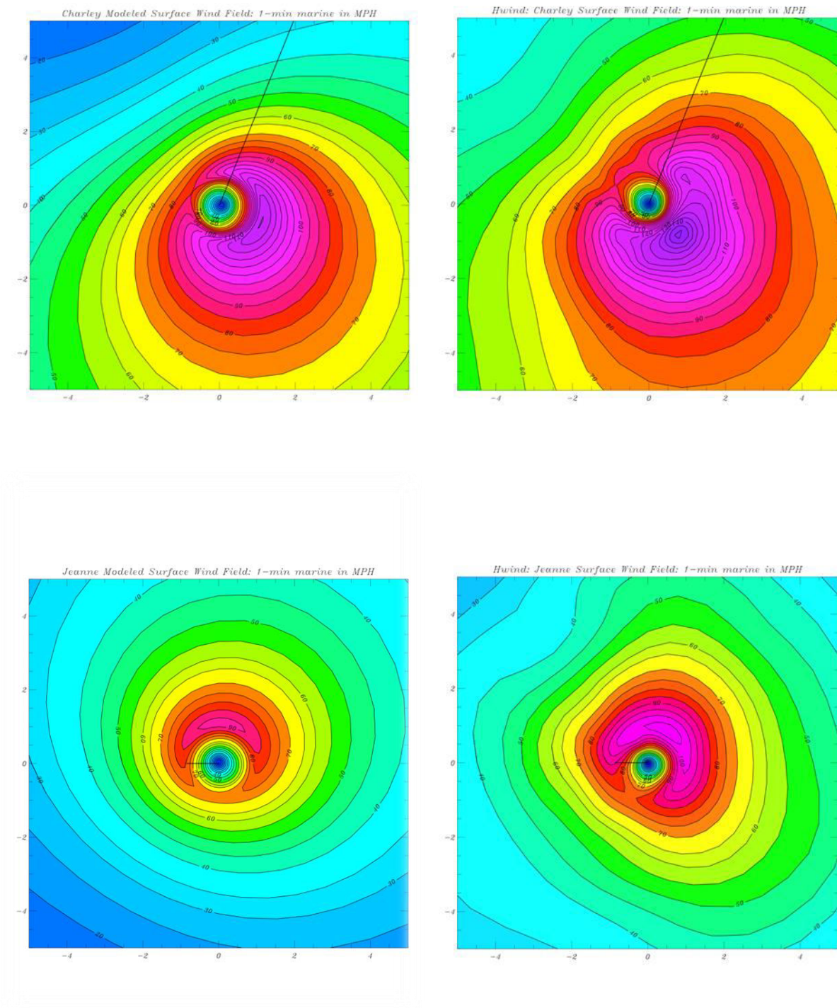
Figure 25. Comparison of modeled (left) and observed (H*Wind, right) landfall wind fields of Hurricane Charley (2004, top) and Hurricane Jeanne (2004, bottom). Line segment indicates storm heading. Horizontal coordinates are in units of R/R_{max} and winds units of miles per hour. All wind fields are for marine exposure.
