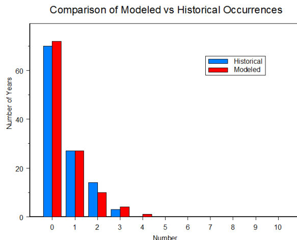
Figure 36. Comparison of modeled vs. historical occurrences.
