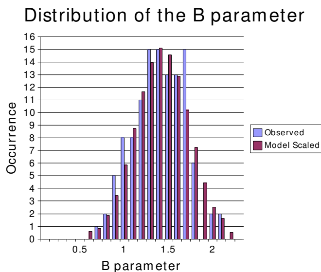
Figure 37. Comparison between the modeled and observed Willoughby and Rahn (2004) B data set.
