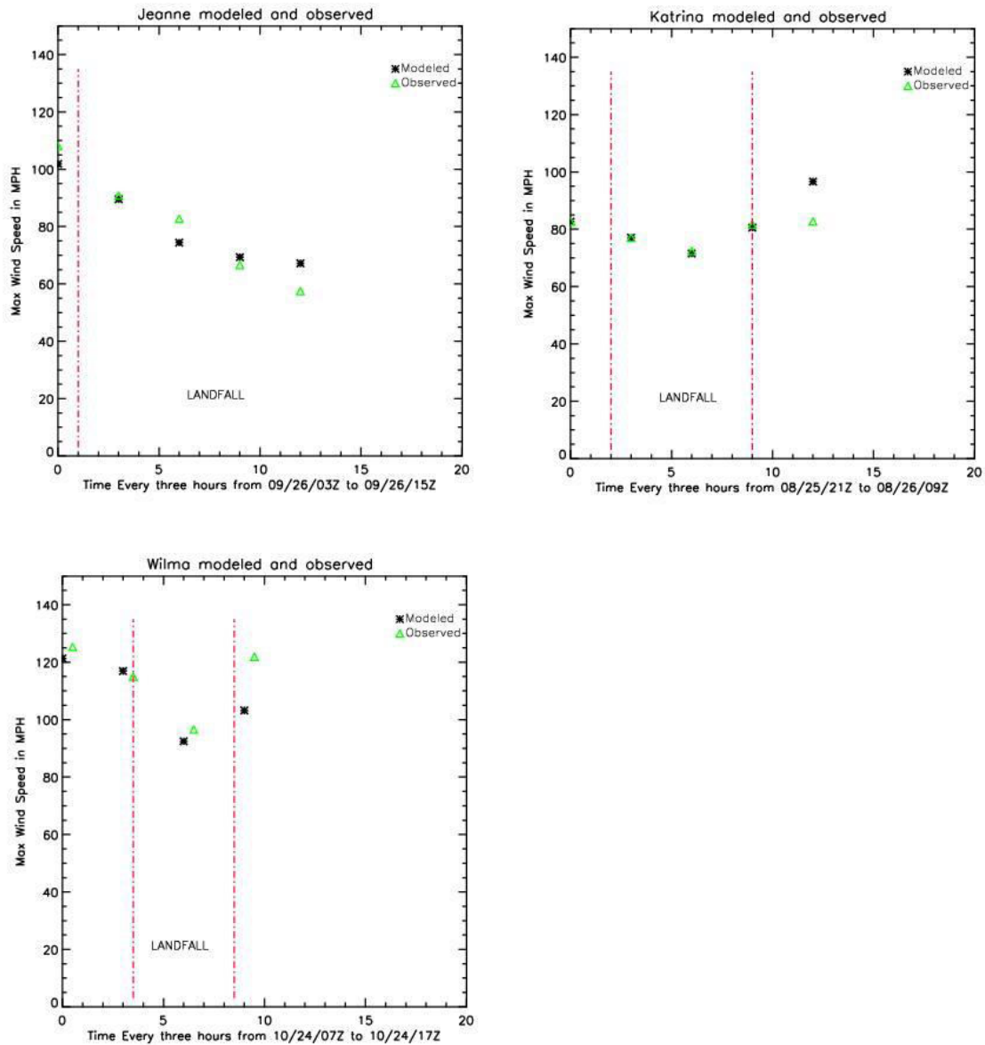
Figure 28. Observed (green) and modeled (black) maximum sustained surface winds as a function of time for Hurricanes Jeanne (2004, top left), Katrina (2005 in South Florida, top right), and Wilma (2005, lower left). Landfall is represented by the vertical dash-dot red line at the left and time of exit as the red line on the right.
