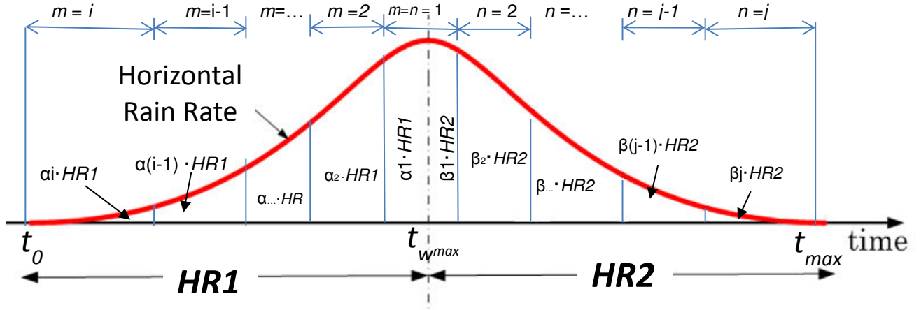
Figure 63. Horizontal rain rate as a function of storm duration.
