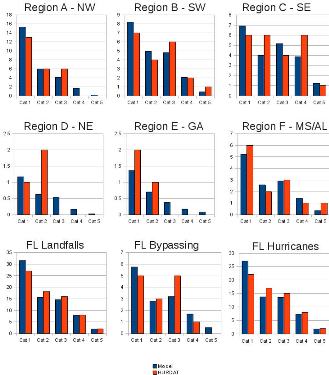
Figure 29. Form M-1 comparison of modeled and historical landfalling hurricane frequency (storms occurring in 114 years) for Regions A–F, FL statewide landfalls (one per FL region), FL bypassing storms, and FL state-wide hurricanes.
