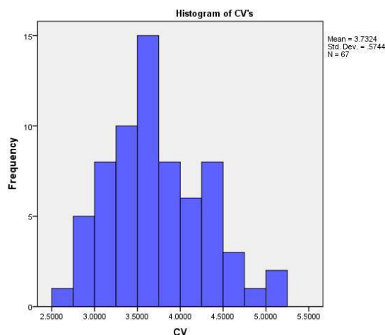
Figure 40. Histogram of CVs for all counties combined.
