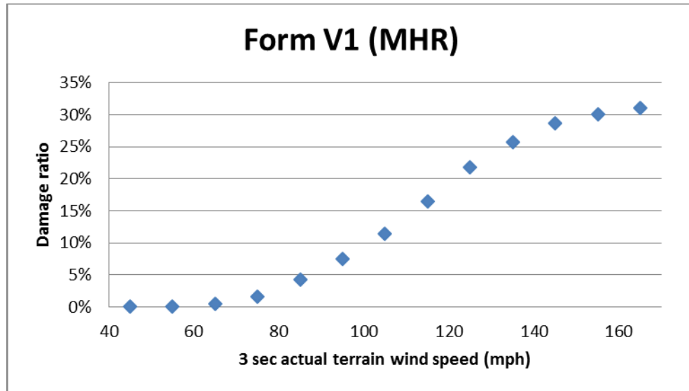
Figure 73. Structure damage vs. 3 sec actual terrain wind speed.
