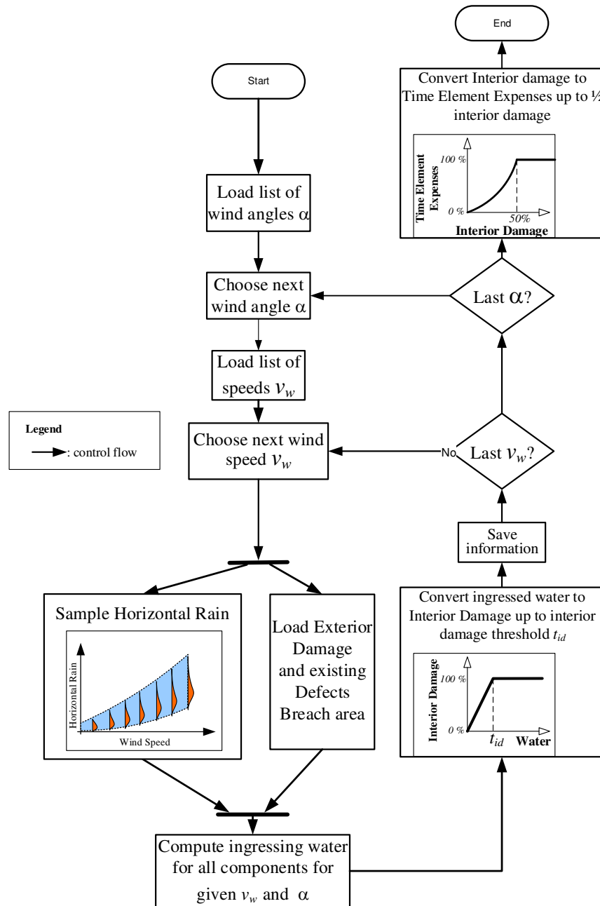
Figure 66. Derivation of time related expenses vulnerabilities for CR.
