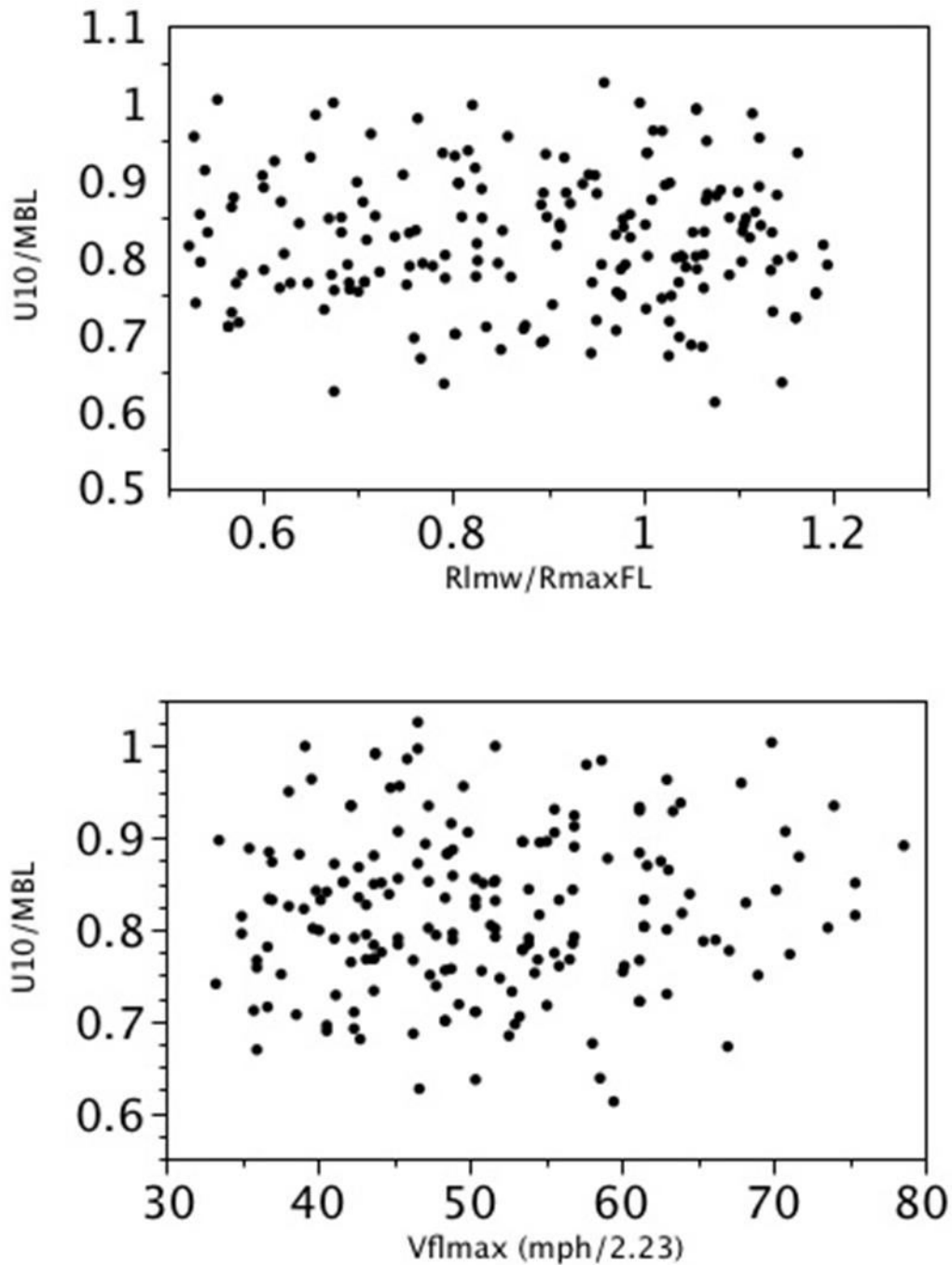
Figure 22. Analysis of 742 GPS dropsonde profiles launched from 2-4 km with flight-level winds at launch greater than hurricane force and with measured surface winds. Upper figure: Dependence of the ratio of 10 m wind speed ( U10 ) to the mean boundary layer wind speed ( MBL ) on the scaled radius (ratio of radius of last measured wind ( R_{lmw} ) to the radius of maximum wind at flight level ( R_{maxFL} )). Lower figure: Surface wind factor ( U10/MBL ) dependence on maximum flight level wind speed ( V_{flmax} , in units of miles per hour / 2.23).
