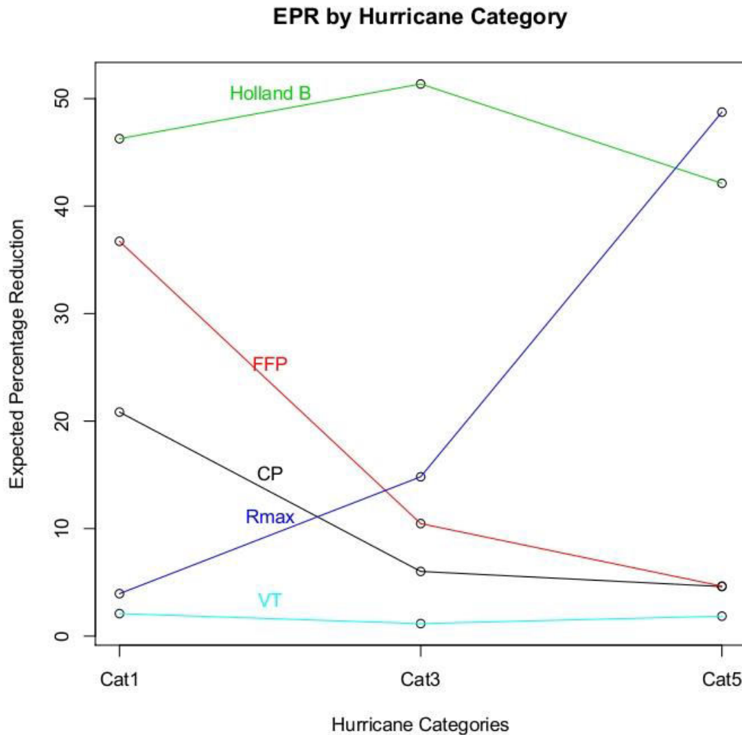
Figure 42. EPRs for Expected Loss Cost for all Input Variables for all Hurricane Categories.
