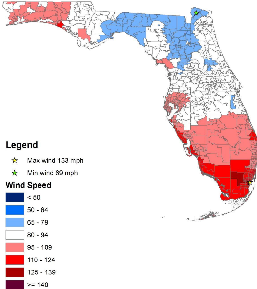
Figure 30. Maximum ZIP Code wind speed for open terrain wind exposure based on simulations of the historical storm set.
