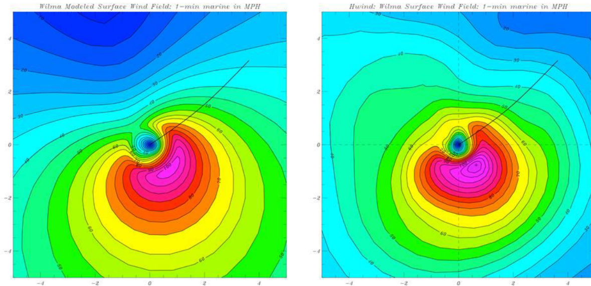
Figure 26. As in Fig. 25 but for Hurricane Wilma of 2005.
