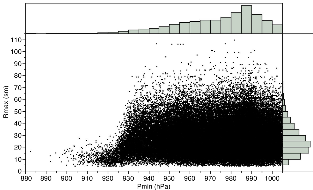
Figure 34. Representative scatter plot of the model input radius of maximum wind (y axis) versus minimum sea-level air pressure at landfall (mb). Relative histograms for each quantity are also shown.
