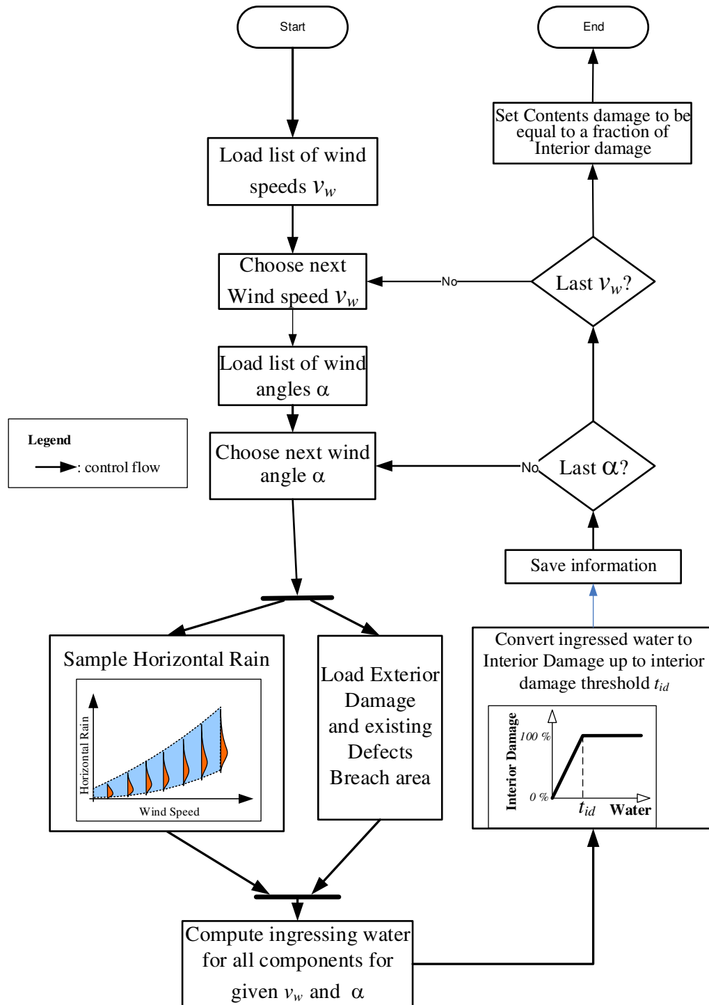
Figure 65b. Derivation of contents vulnerabilities for CR.
