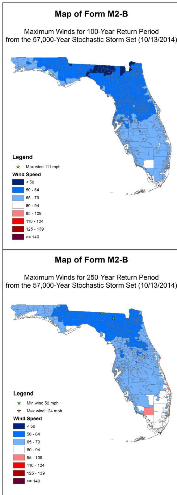
Figure 33. 100- and 250-year return period wind speeds at Florida ZIP Codes for actual terrain wind exposure. Note that winds below 50 mph were not saved for this calculation, and thus the minimum wind cannot be determined.
