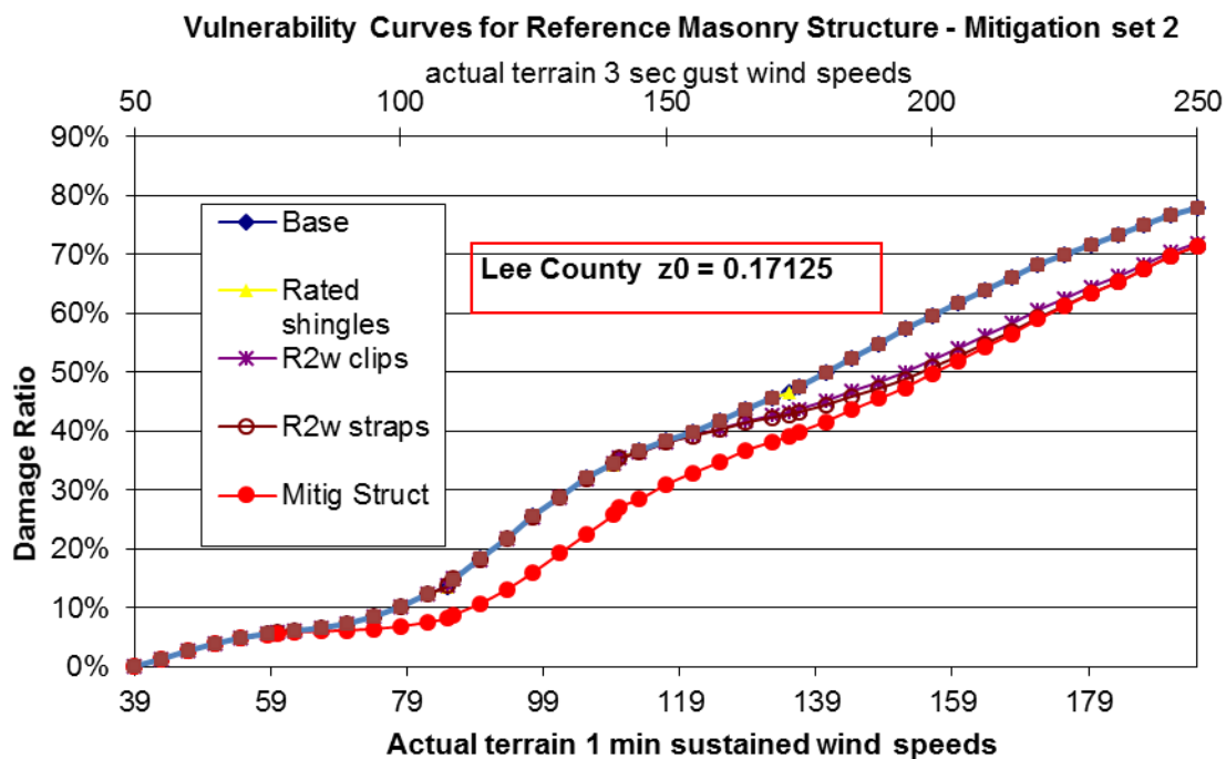
Figure 75. Mitigation measures for masonry homes.
