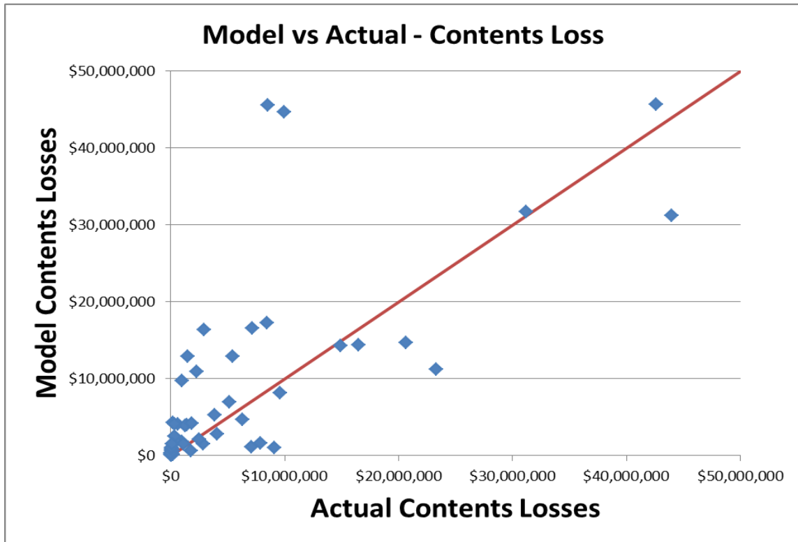
Figure 67. Model vs. Actual-Contents Loss.
