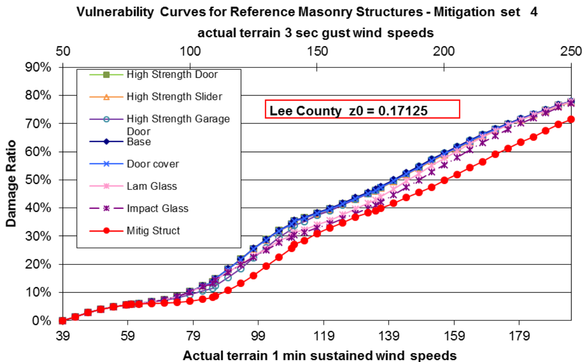
Figure 76. Mitigation measures for masonry homes.
