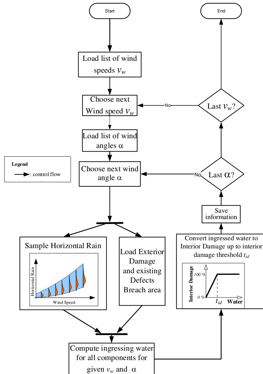
Figure 62. Flowchart of the interior damage model.
