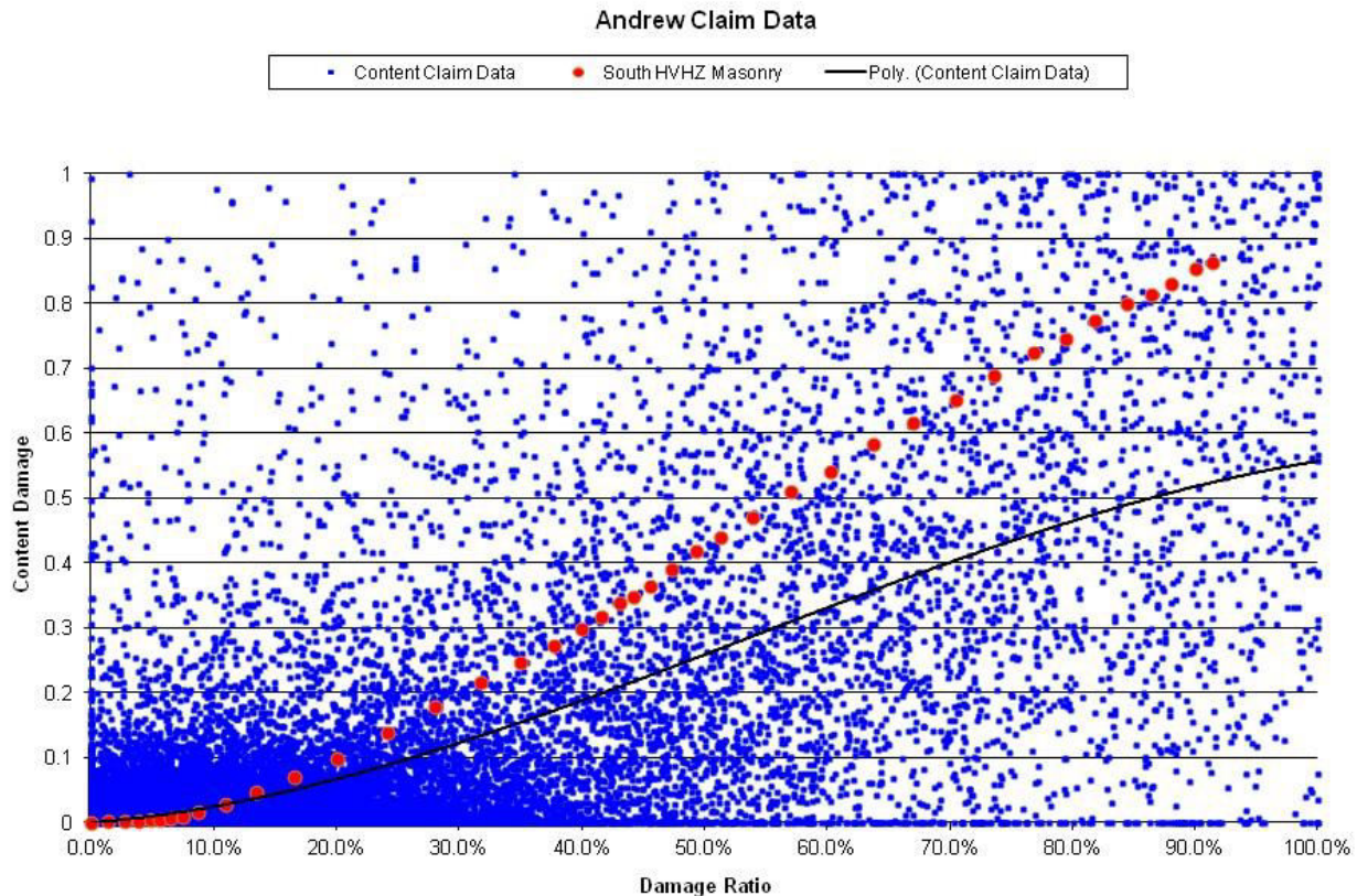
Figure 79. Modeled vs. actual relationship between structure and content damage ratios for Hurricane Andrew.
