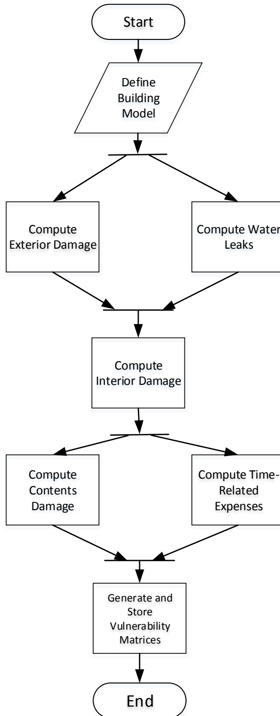
Figure 65a. Derivation of contents and additional living expenses vulnerabilities for PR.
