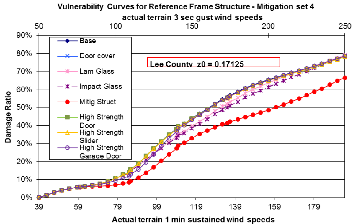
Figure 78. Mitigation measures for frame homes.
