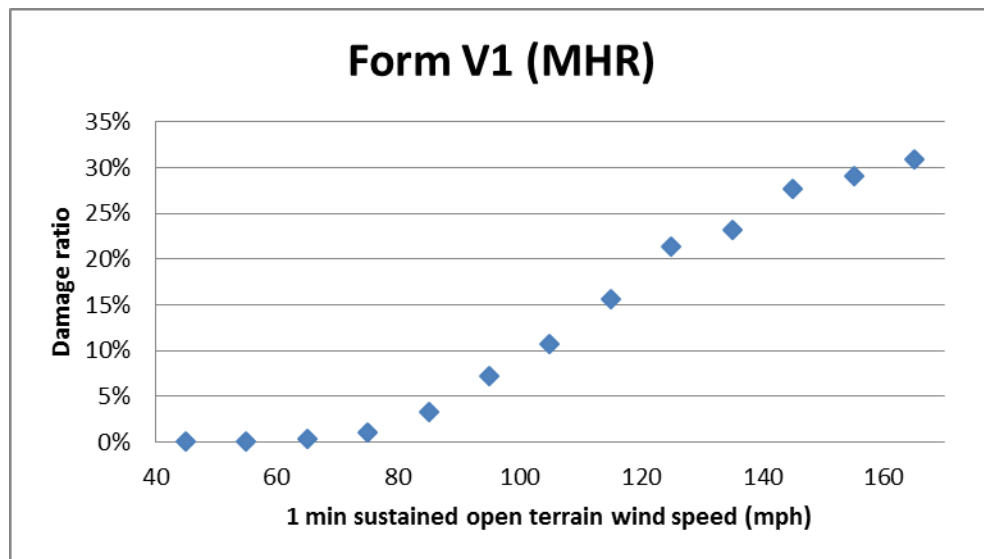
Figure 74. Structure damage vs. 1 minute sustained wind speed.
