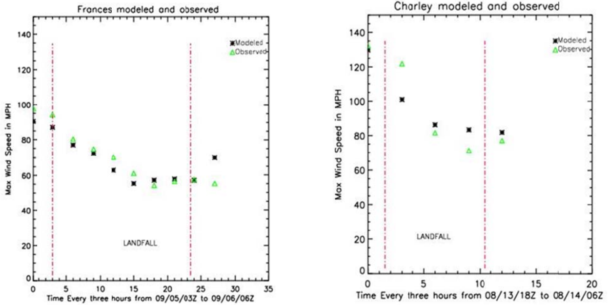
Figure 3534. Observed (green) and modeled (black) maximum sustained surface winds as a function of time for 2004 Hurricanes Frances (left) and Charley (right). Landfall is represented by the vertical dash-dot red line at the left and time of exit as the red line on the right.
