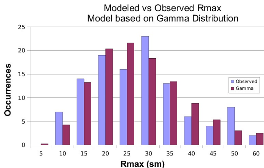
Figure 2728. Comparison of observed landfall R_{max} (sm) distribution to a gamma distribution fit of the data.
