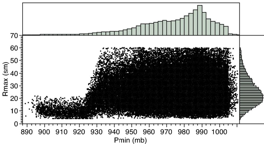
Figure 4241. Representative scatter plot of the model input radius of maximum wind (y axis) versus minimum sea-level air pressure at landfall (mb). Relative histograms for each quantity are also shown.
