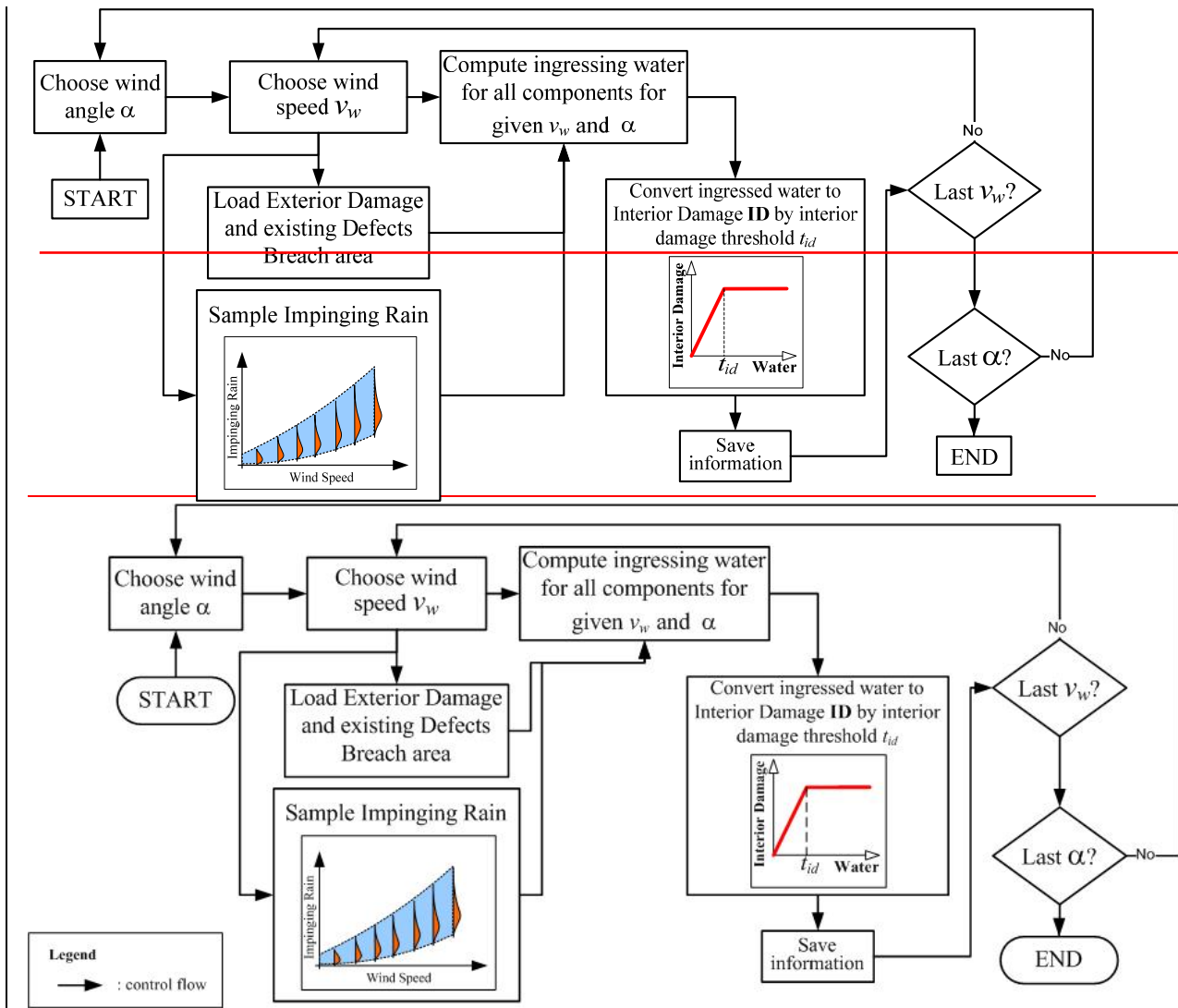
Figure 16. Flowchart of the interior damage model.
