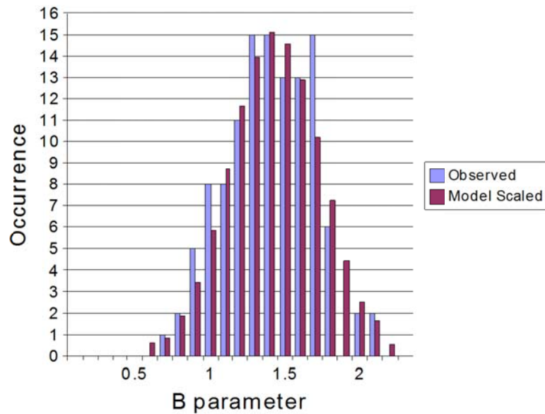
Figure 8685. Comparison between the modeled and observed Willoughby and Rahn (2004) B data set.
