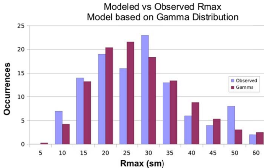
Figure 8786. Observed and expected distribution using a gamma distribution.
