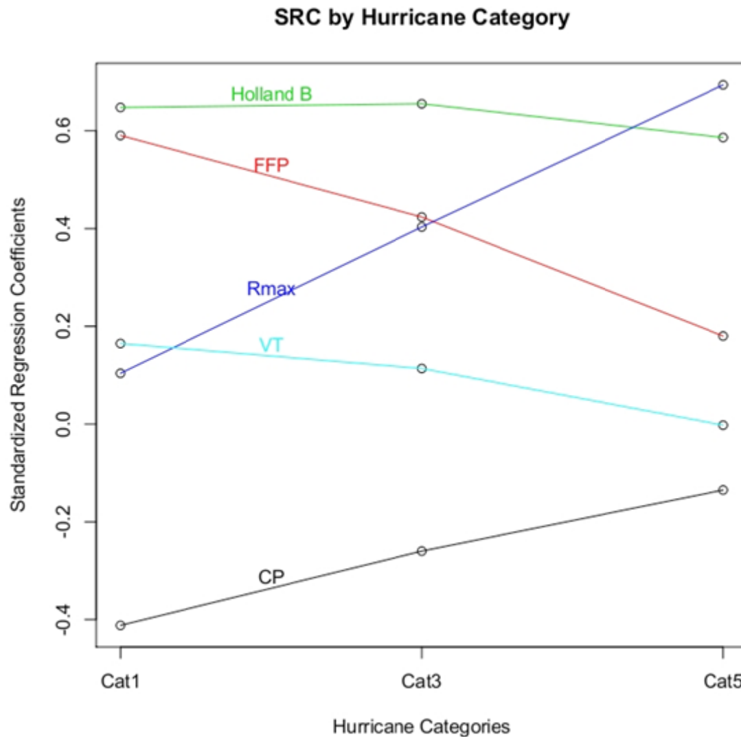
Figure 9089. SRCs for expected loss cost for all input variables for all hurricane categories.
