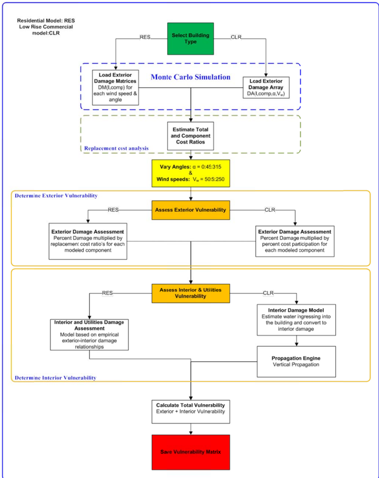
Figure 4544. Procedure to create vulnerability matrix.
