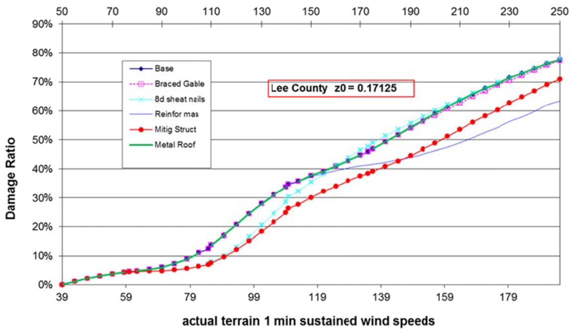
Vulnerability Curves for Reference Masonry Structure - Mitigation set 1 actual terrain 3 sec gust wind speeds
