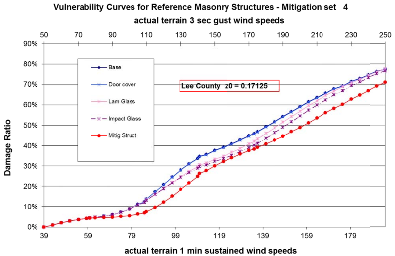
Figure 6463. Mitigation measures for masonry homes.
