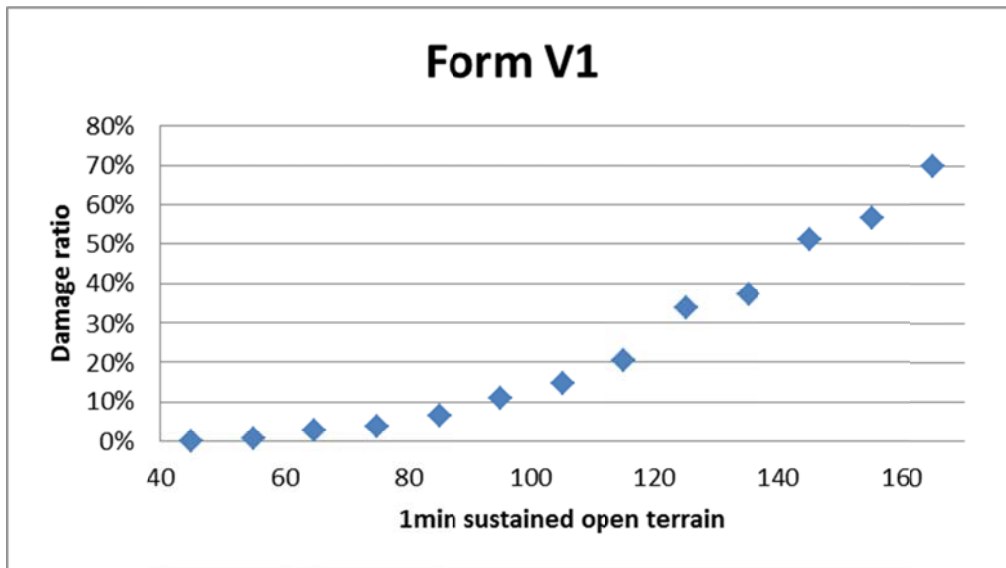
Figure 6059. Structure damage vs. 1 minute sustained wind speed.
