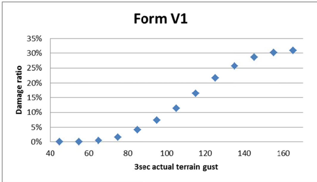
Figure 6160. Structure damage vs. 3 sec actual terrain wind speed.
