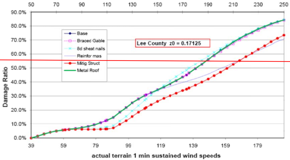
Vulnerability Curves for Reference Masonry Structure - Mitigation set 1 actual terrain 3 sec gust wind speeds
