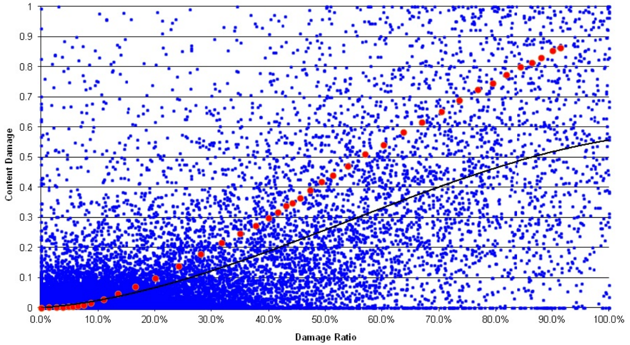
Figure 5655. Modeled vs. actual relationship between structure and content damage ratios for Hurricane Andrew.
