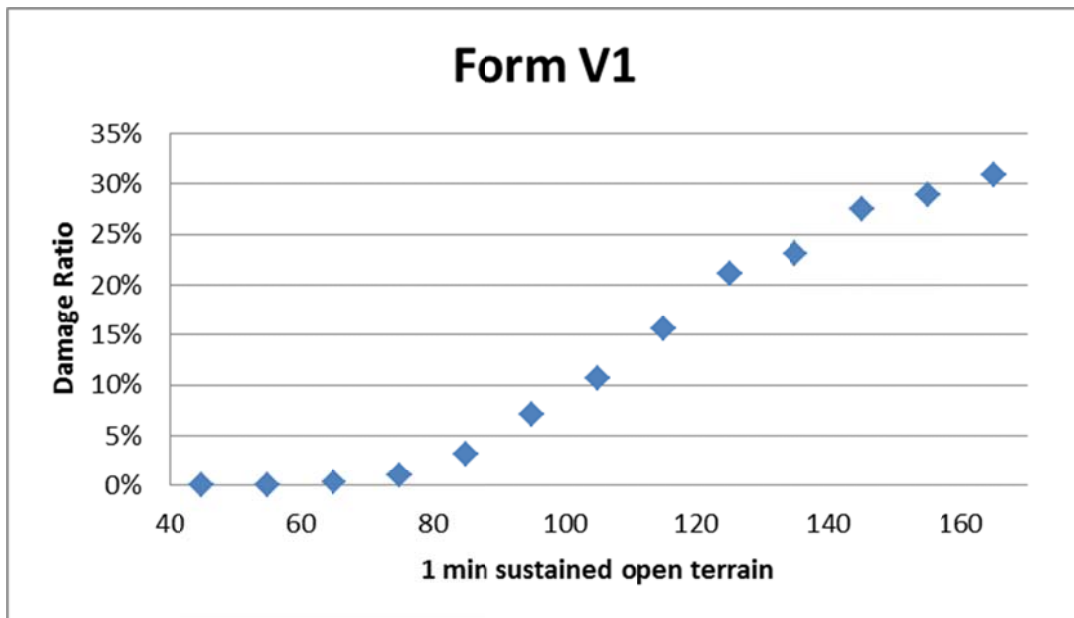
Figure 6261. Structure damage vs. 1 minute sustained wind speed.
