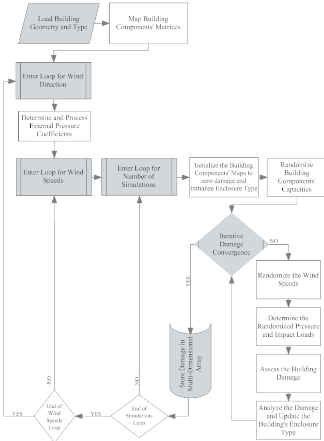
Figure 4443. Monte Carlo simulation procedure to predict damage.
