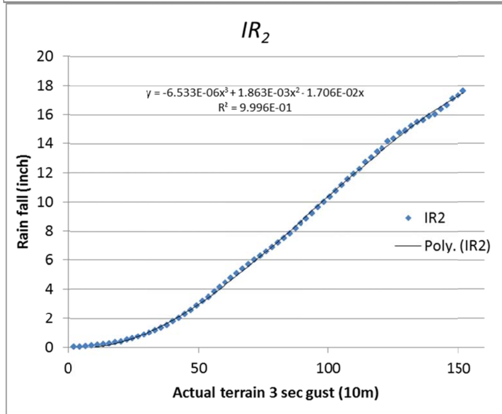
Figure-4847. Mean accumulated impinging rain as a function of peak 3-second wind gust.
