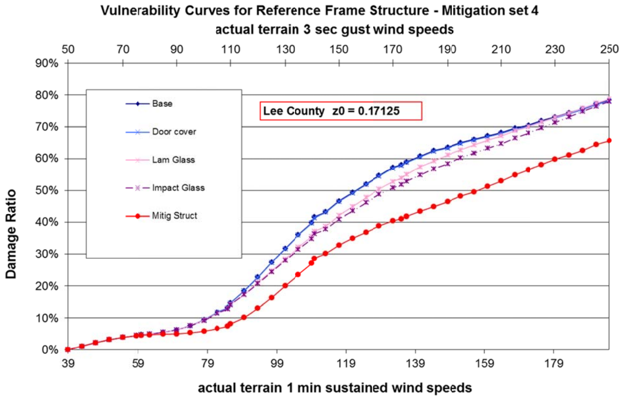
Figure 6665. Mitigation measures for frame homes.
