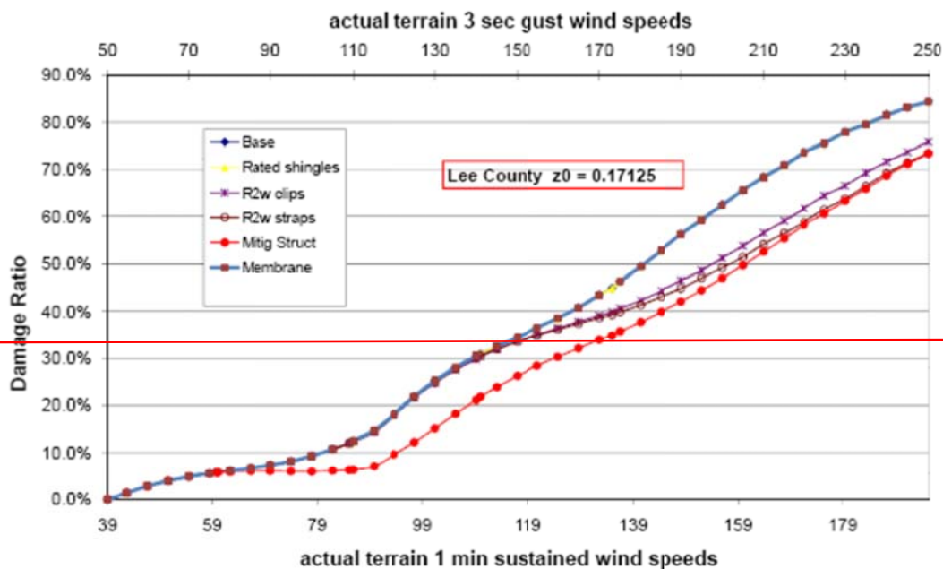
Vulnerability Curves for Reference Masonry Structure - Mitigation set 2
