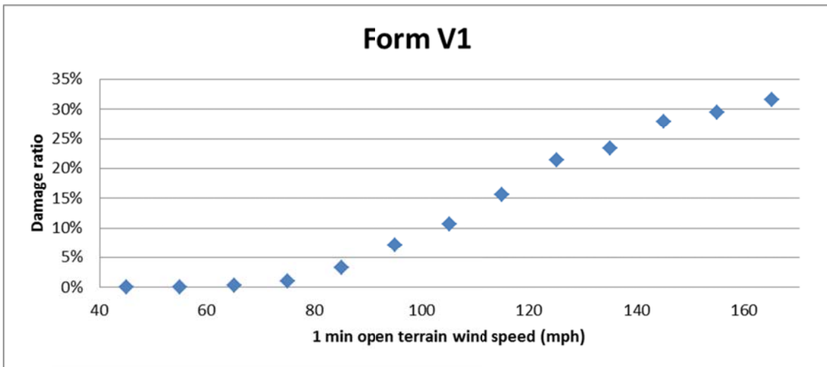
Figure 5857. Structure damage vs. 1 minute sustained wind speed.
