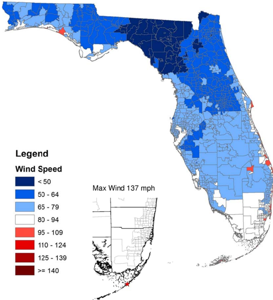
Figure 3839. Maximum ZIP Code wind speed for actual terrain wind exposure based on simulations of the historical storm set.
