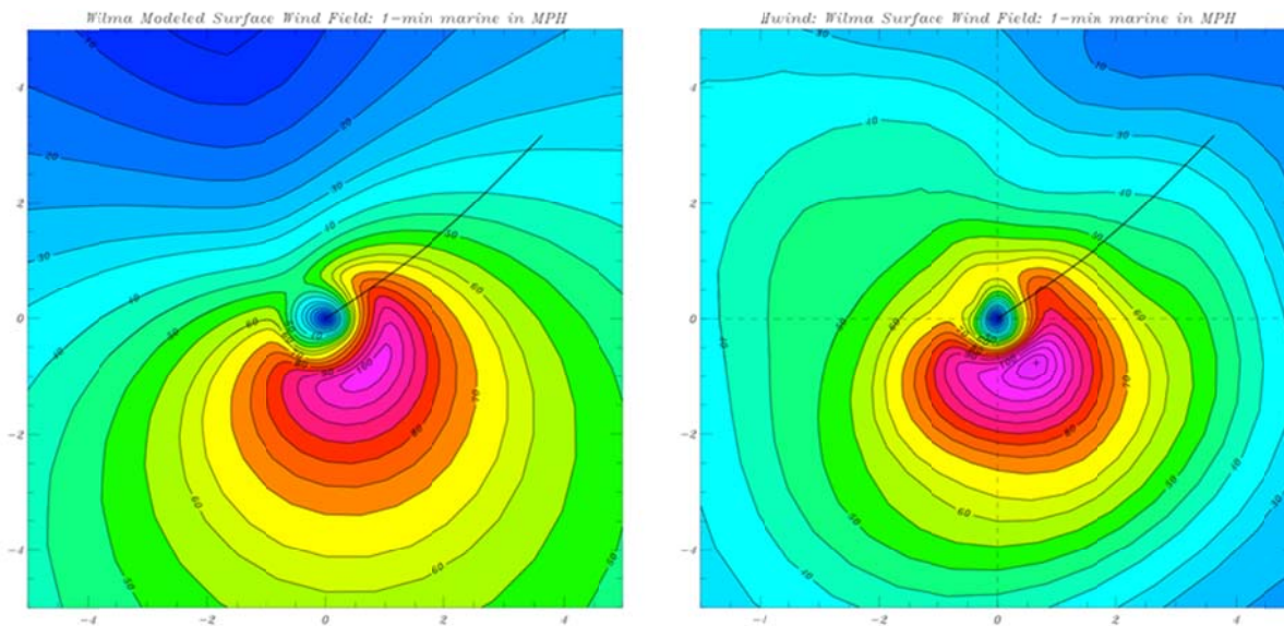
Figure 3433. As in Fig. 33 but for Hurricane Wilma of 2005.
