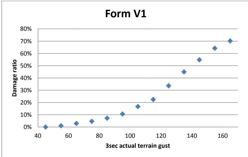
Figure 5958. Structure damage vs. 3 sec actual terrain wind speed.
