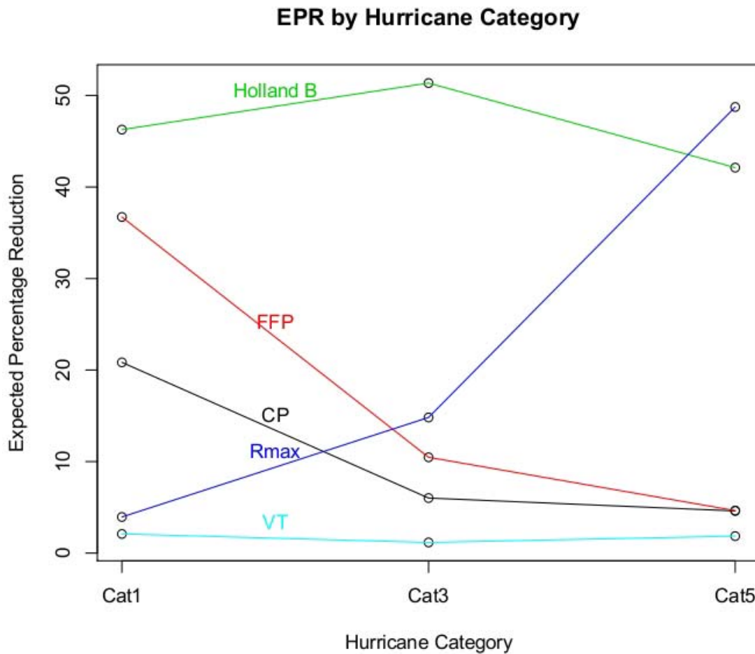
Figure 103-104. EPRs for Expected Loss Cost for all Input Variables for all Hurricane Categories.
