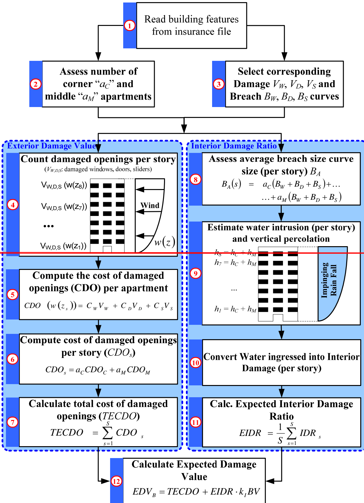
Figure 4645. Exterior and interior damage assessment for MHB.
