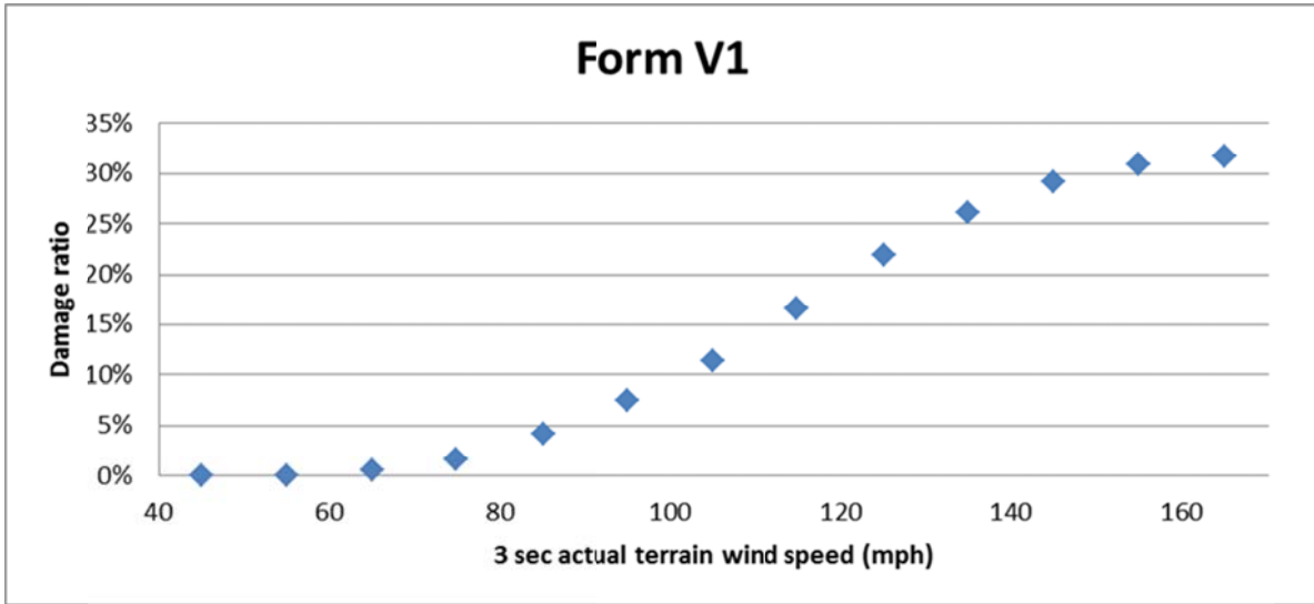
Figure 5756. Structure damage vs. 3 sec actual terrain wind speed.
