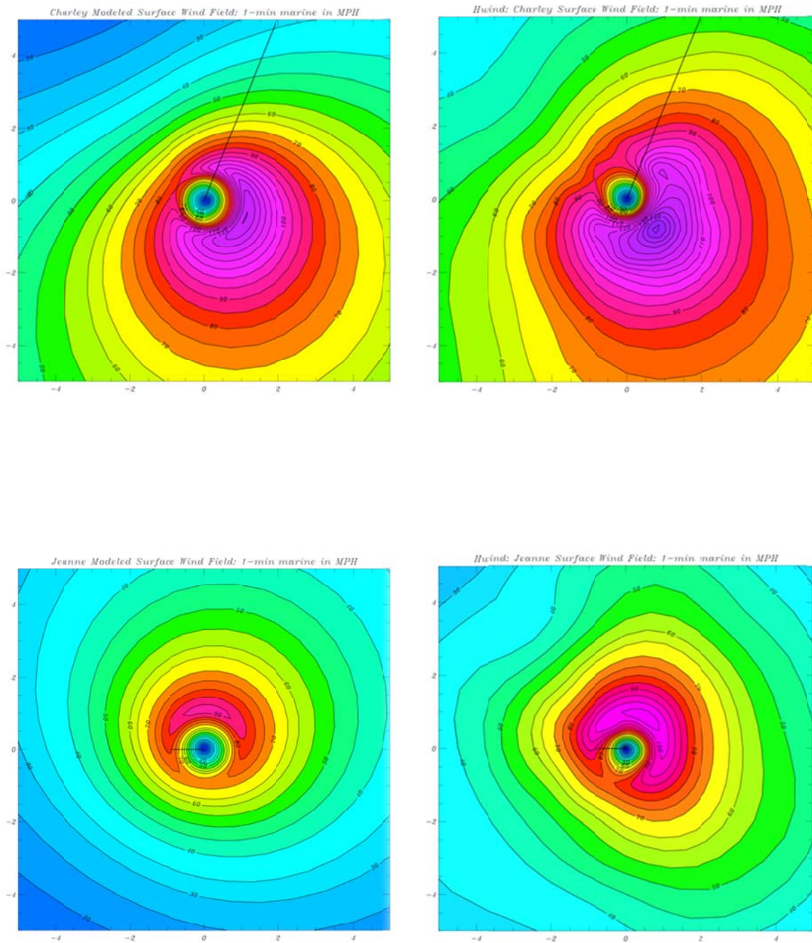
Figure-3332. Comparison of modeled (left) and observed (H*Wind, right) landfall wind fields of Hurricane Charley (2004, top) and Hurricane Jeanne (2004, bottom). Line segment indicates storm heading. Horizontal coordinates are in units of R/R_{max} and winds units of miles per hour. All wind fields are for marine exposure.
