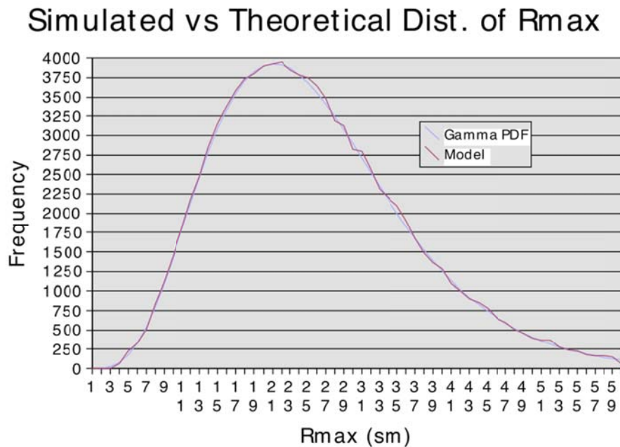
Figure 6. Comparison of 100,000 Rmax values sampled from the gamma distribution for Category 1–4 storms to the expected values.
