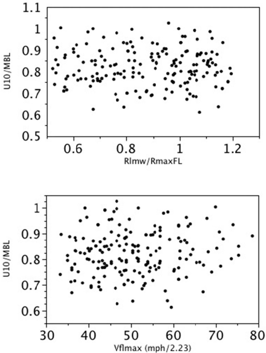
Figure 3029. Analysis of 742 GPS dropsonde profiles launched from 2-4 km with flight-level winds at launch greater than hurricane force and with measured surface winds. Upper figure: Dependence of the ratio of 10 m wind speed ( U_{10} ) to the mean boundary layer wind speed (MBL) on the scaled radius (ratio of radius of last measured wind ( R_{lmw} ) to the radius of maximum wind at flight level ( R_{maxFL} )). Lower figure: Surface wind factor ( U_{10}/MBL ) dependence on maximum flight level wind speed ( V_{flmax} , in units of miles per hour / 2.23).
