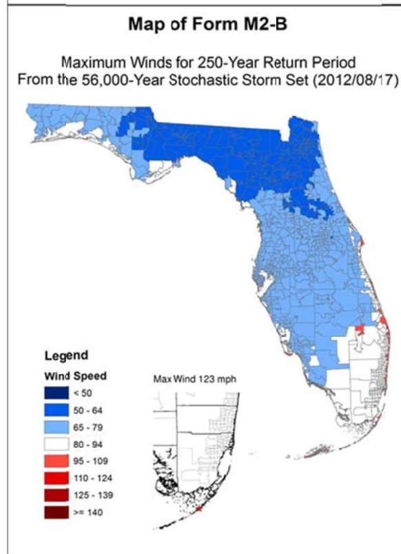
Figure-4140. 100- and 250-year return period wind speeds at Florida ZIP Codes for actual terrain wind exposure.
