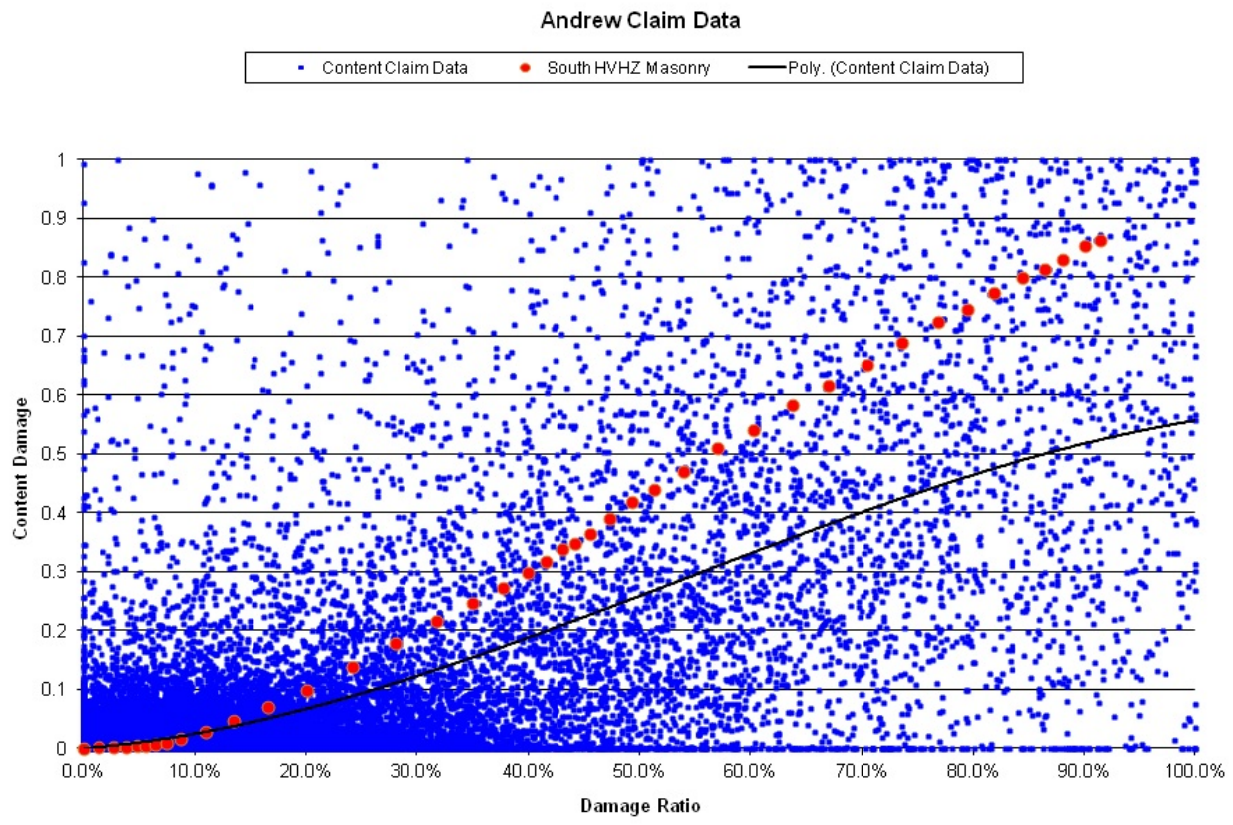
Figure 6667. Modeled vs. actual relationship between structure and content damage ratios for Hurricane Andrew.
