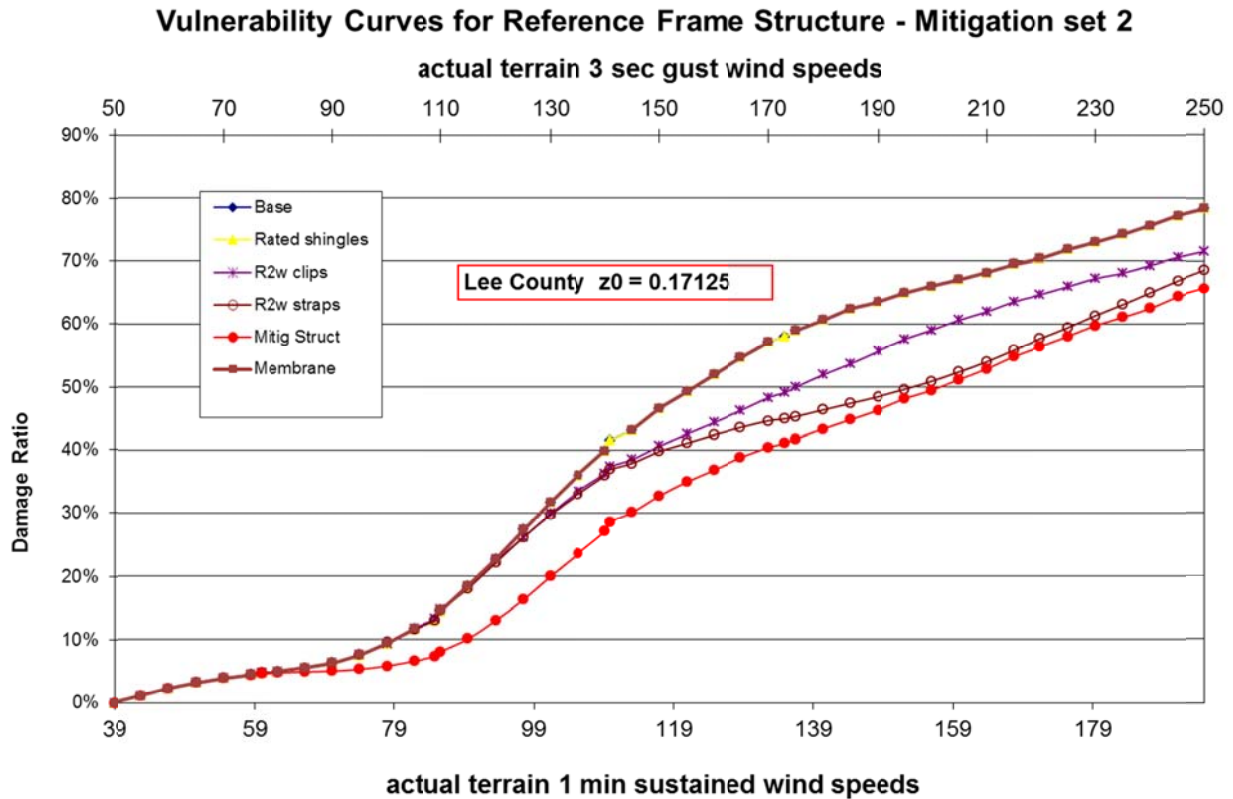
Figure 6564. Mitigation measures for frame homes.
