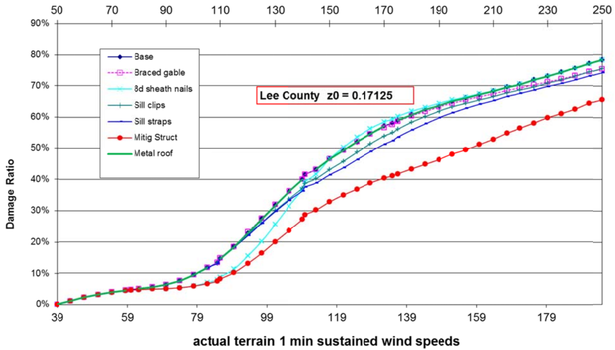
Vulnerability Curves for Reference Frame Structure - Mitigation set 1 actual terrain 3 sec gust wind speeds
