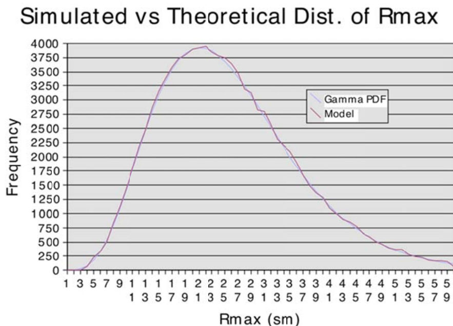
Figure 289. Comparison of 100,000 R_{max} values sampled from the gamma distribution for Cat 1–4 storms to the expected values.
