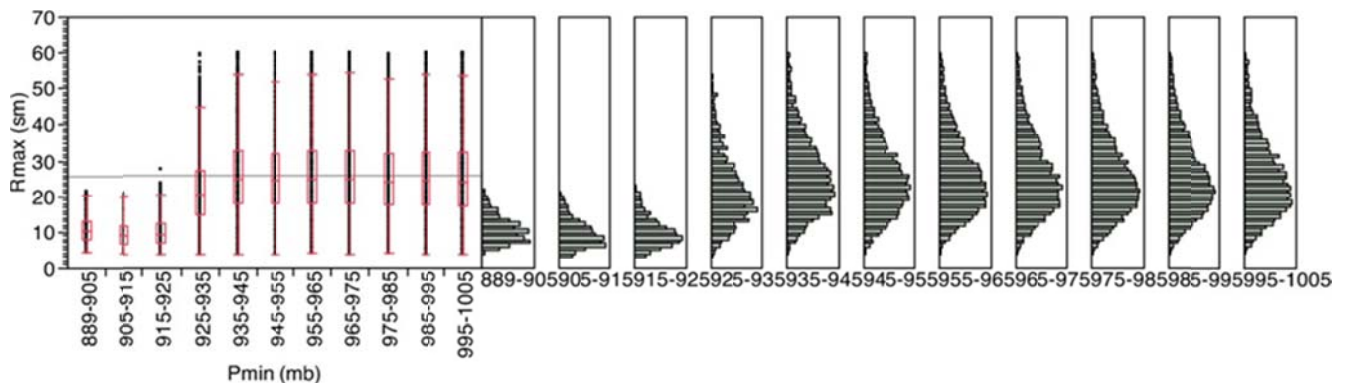
Figure 4342. One way box plot (left) of R_{max} (continuous) response across 10 mb P_{min} groups. Boxes (and whiskers) are in red; standard deviations are in blue. Histograms (right) for each P_{min} group.
