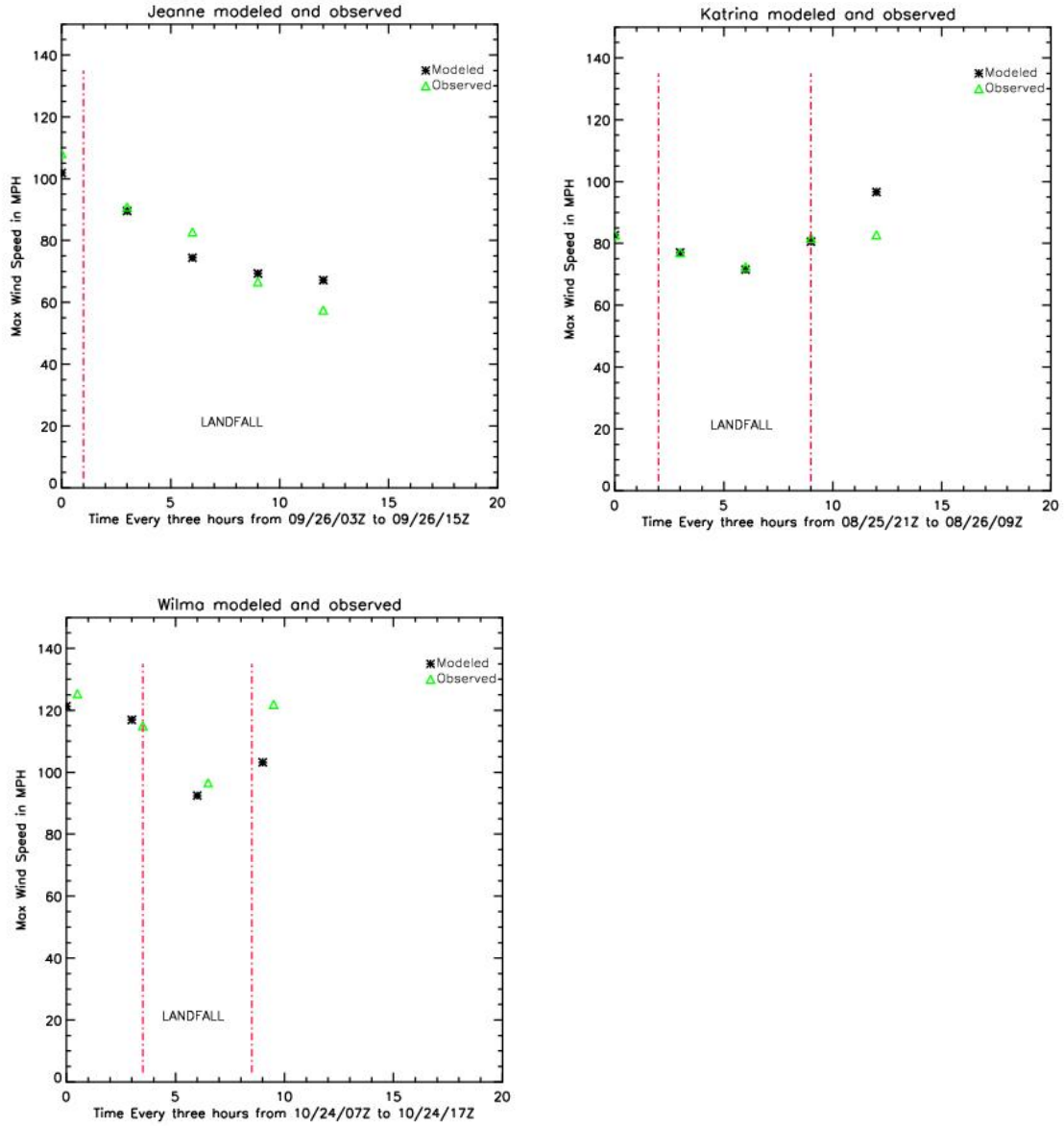
Figure 3536. Observed (green) and modeled (black) maximum sustained surface winds as a function of time for Hurricanes Jeanne (2004, top left), Katrina (2005 in South Florida, top right), and Wilma (2005, lower left). Landfall is represented by the vertical dash-dot red line at the left and time of exit as the red line on the right.
