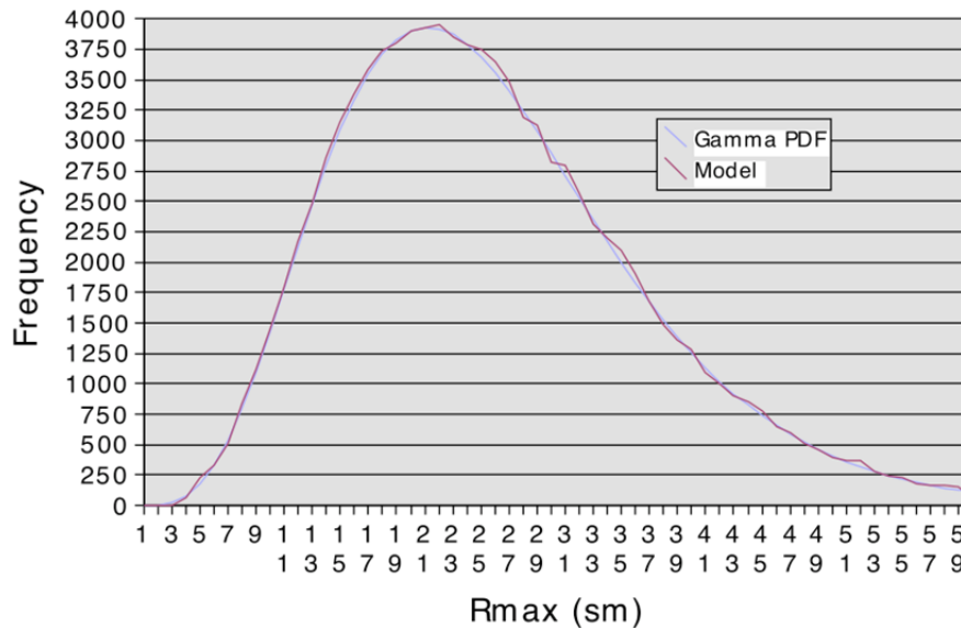
Figure 6. Comparison of 100,000 R_{max} values sampled from the gamma distribution for Category 1–4 storms to the expected values.
