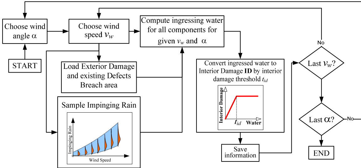
Figure 16. Flowchart of the interior damage model.
