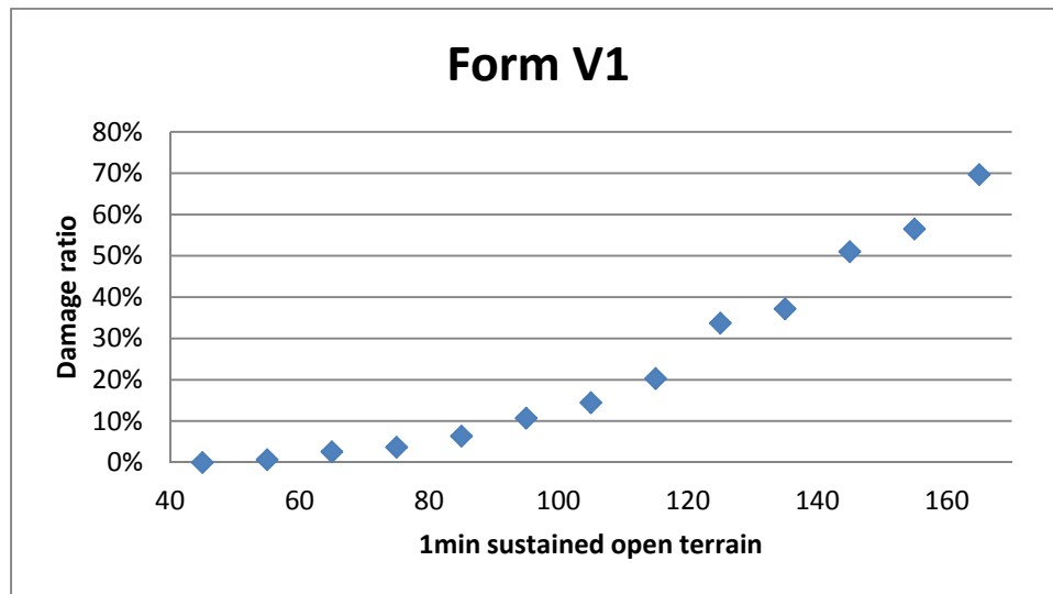
Figure 60. Structure damage vs. 1 minute sustained wind speed.
