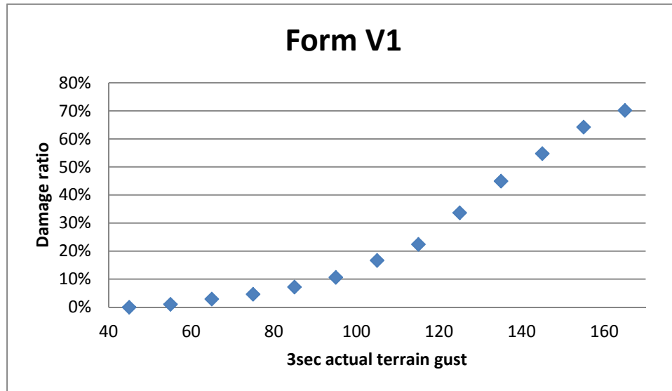
Figure 59. Structure damage vs. 3 sec actual terrain wind speed.
