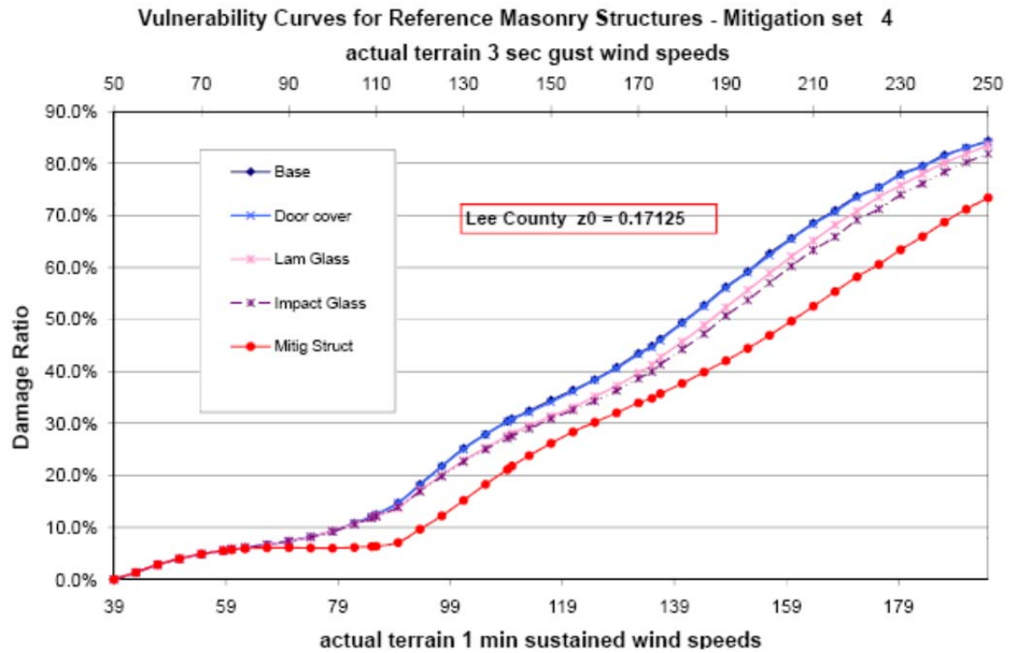
Figure 64. Mitigation measures for masonry homes.
