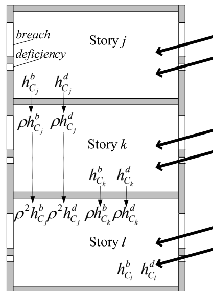
Figure 50: Diagram of water intrusion through breaches, deficiencies and percolation in a 3-story building.
