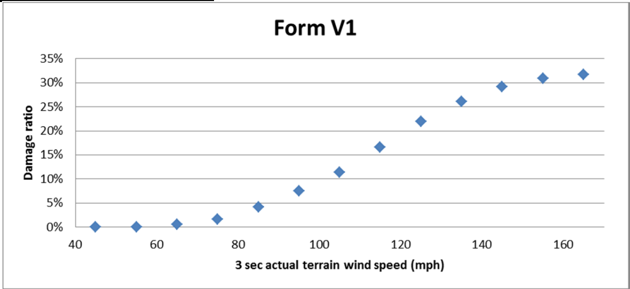
Figure 57. Structure damage vs. 3 sec actual terrain wind speed.
