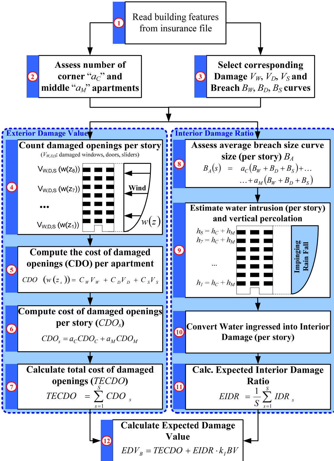
Figure 18. Exterior and interior damage assessment for MHB.
