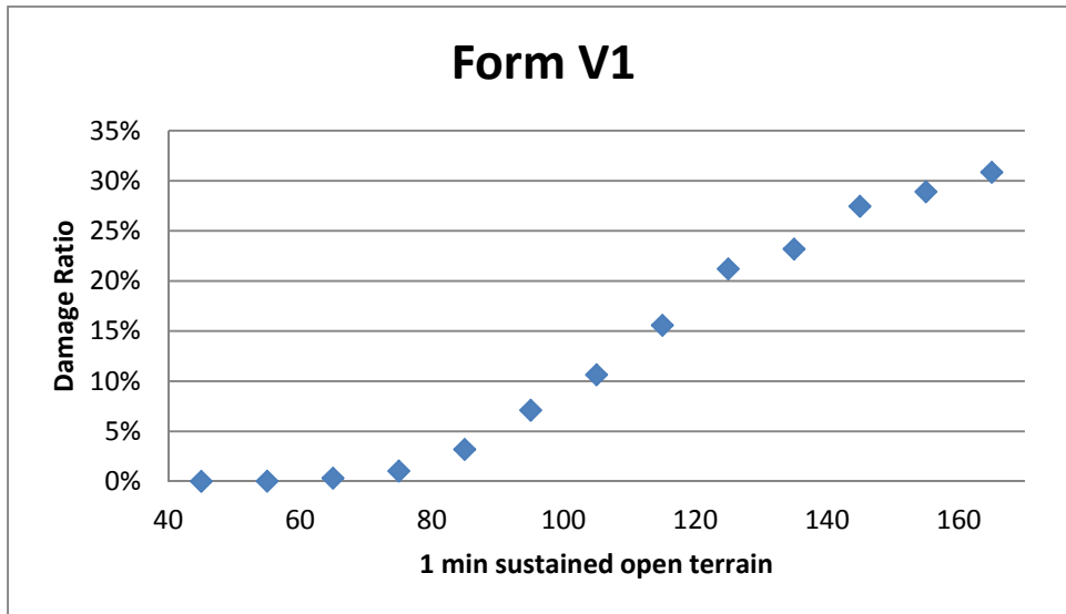
Figure 62. Structure damage vs. 1 minute sustained wind speed.
