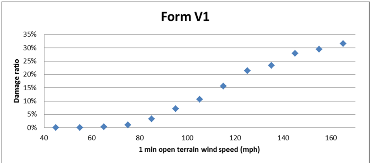
Figure 58. Structure damage vs. 1 minute sustained wind speed.
