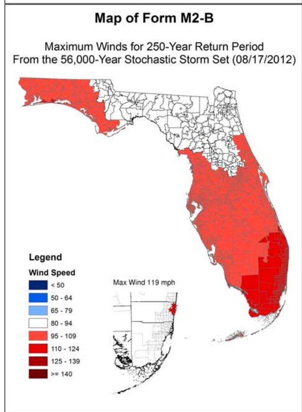
Figure 40. 100- and 250-year return period wind speeds at Florida ZIP Codes for open terrain wind exposure.
