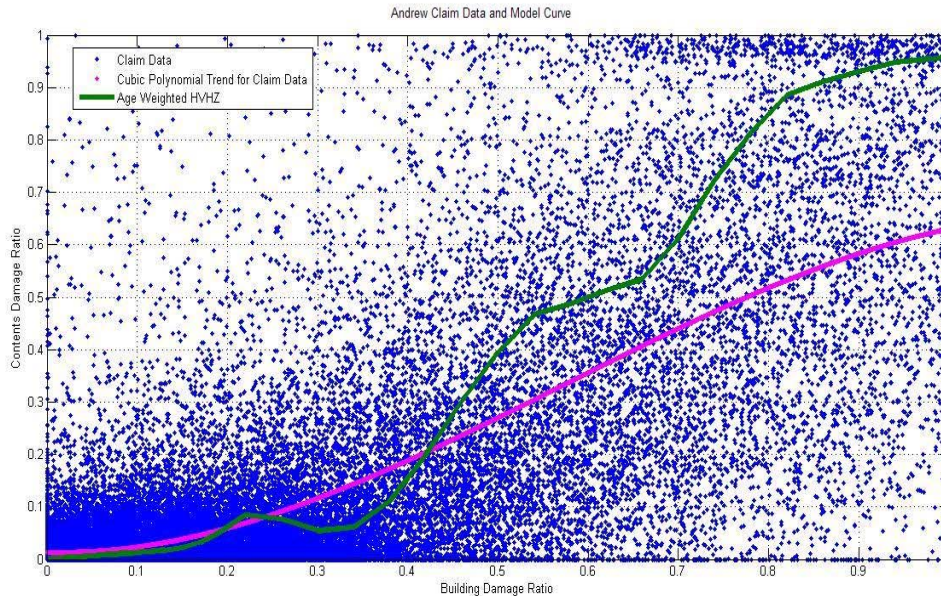
Figure 56. Modeled vs. actual relationship between structure and content damage ratios for Hurricane Andrew.
