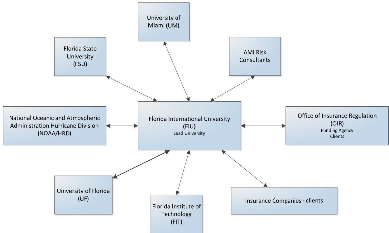
Figure 26. Organizational structure.
