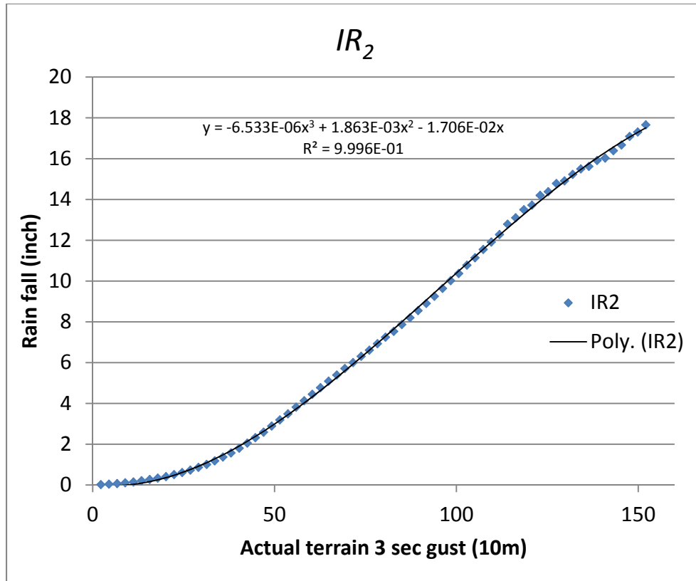
Figure 48. Mean accumulated impinging rain as a function of peak 3-second wind gust.
