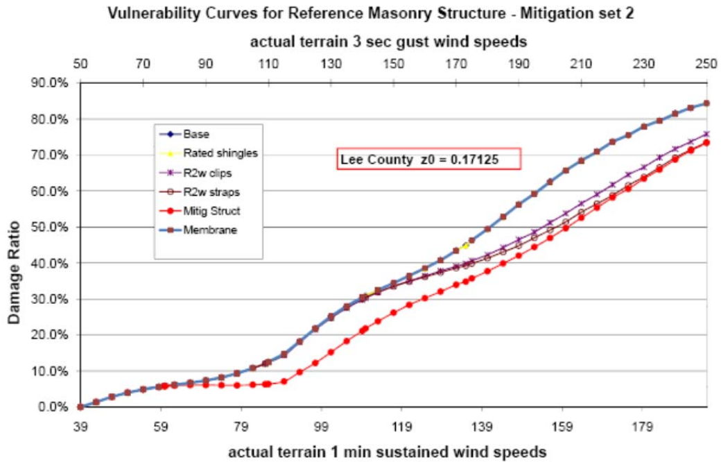
Figure 63. Mitigation measures for masonry homes.
