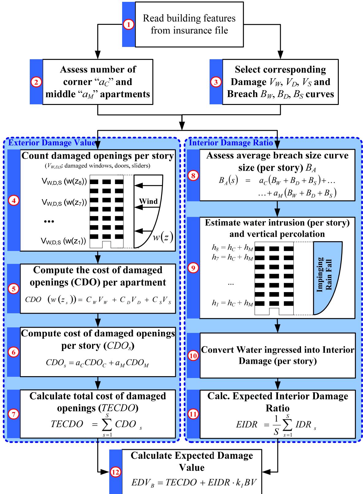
Figure 46. Exterior and interior damage assessment for MHB.
