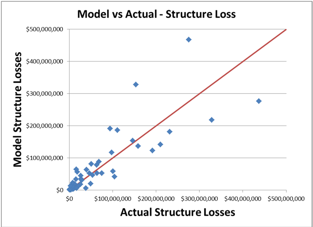
Figure 52. Model vs. Actual—Structure Loss.
