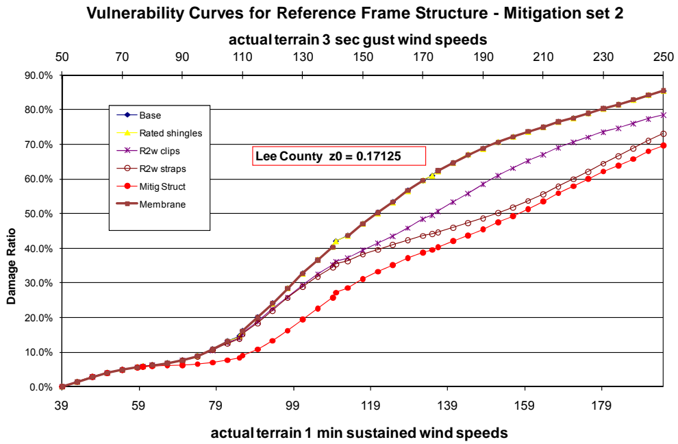
Figure 65. Mitigation measures for frame homes.
