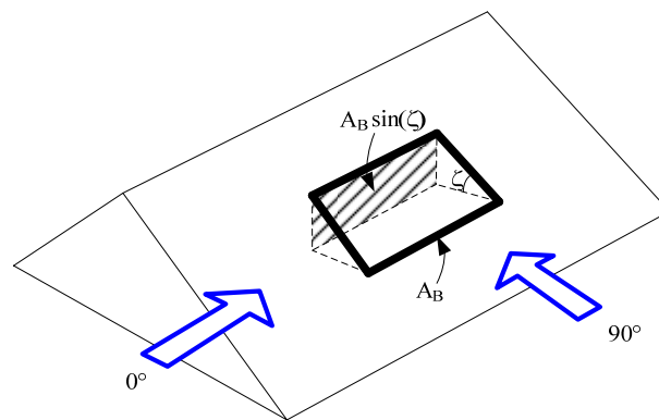
Figure 49: f_{RedRoof} represents the breached roof area that is exposed to impinging rain as a function of wind angle of attack.
