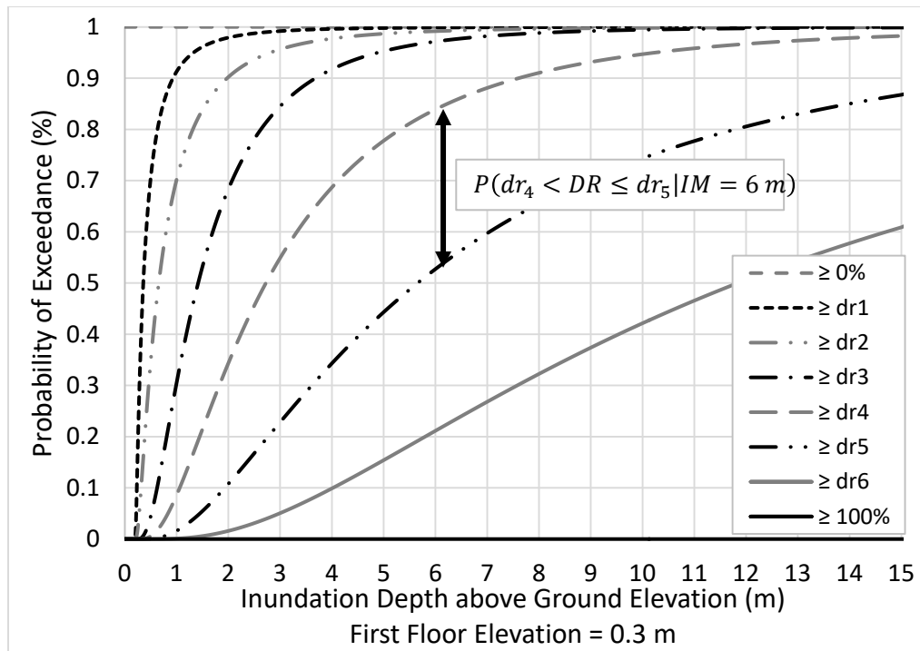
Figure 17. Example of Coastal Flood Fragility Curves.
