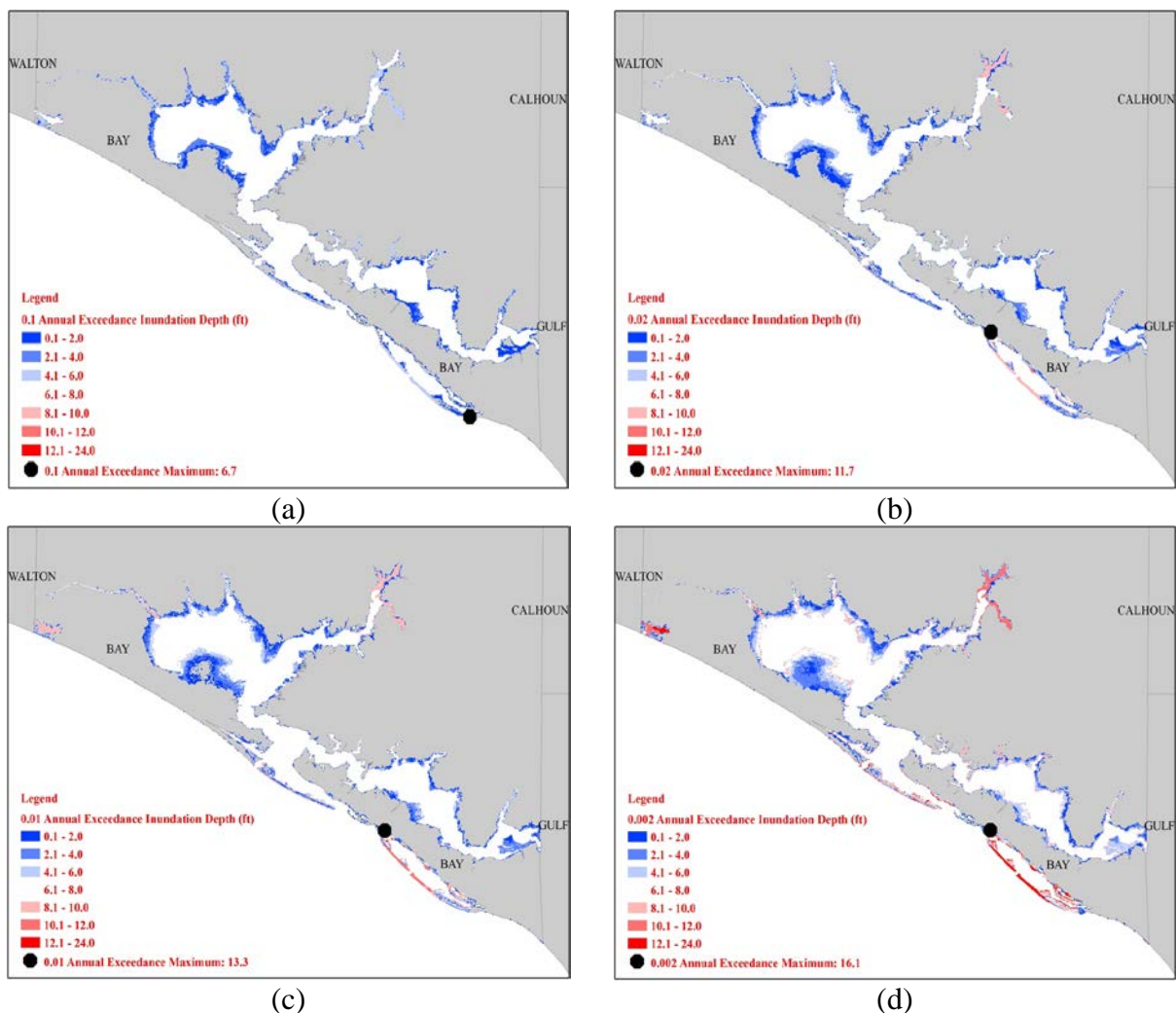
Figure 150. Modeled flood extent and inundation depth corresponding to (a) 0.1, (b) 0.02, (c) 0.01, and (d) 0.002 annual exceedance probability at Bay County (Panhandle)
