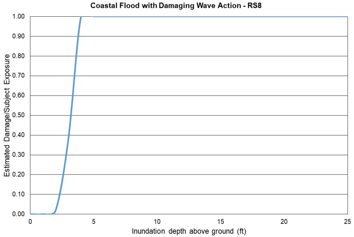
Figure 200. Coastal flood estimated damage vs inundation depth, Reference Building 8.
