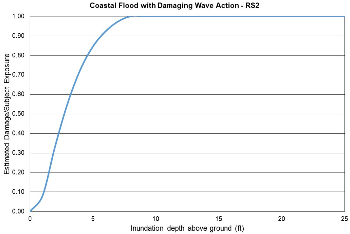
Figure 194. Coastal flood estimated damage vs inundation depth, Reference Building 2.
