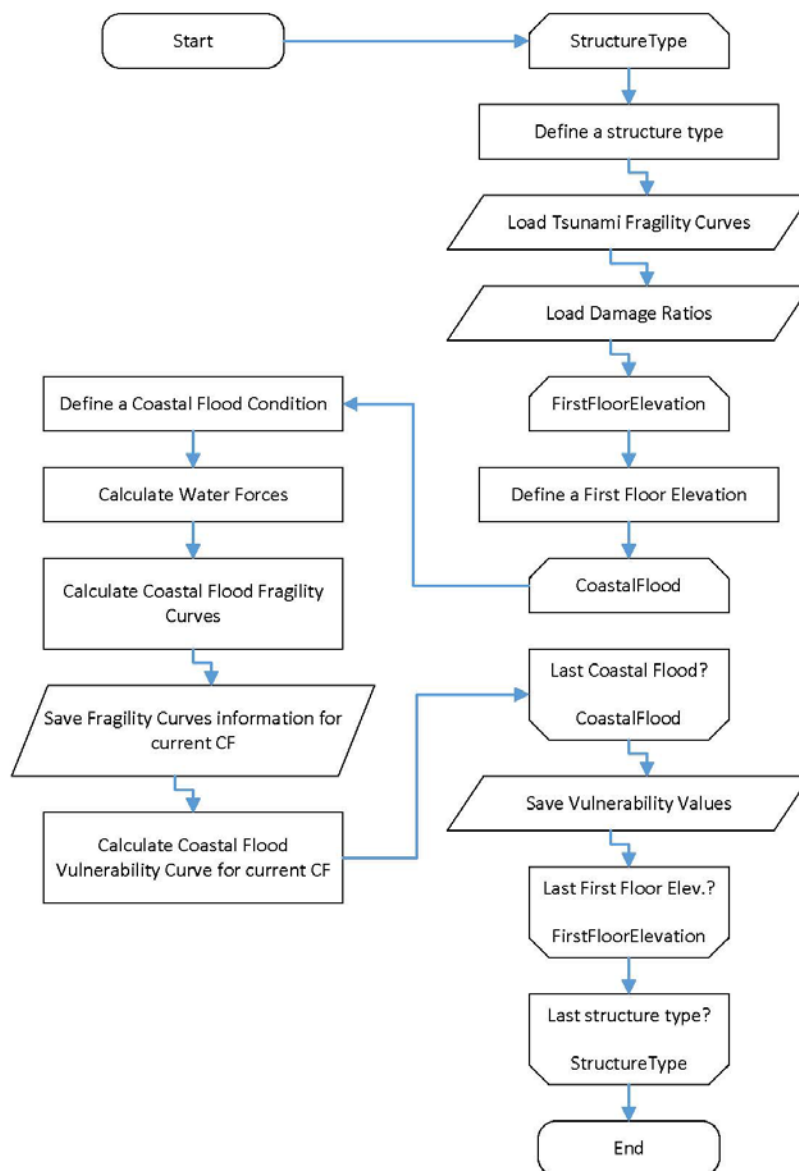
Figure 78. Coastal flood vulnerability for residential structures.
