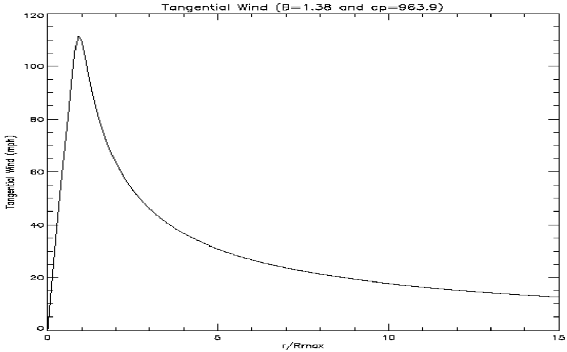
Figure 30. Axisymmetric rotational wind speed (mph) vs. scaled radius for B = 1.38 , \text{DeIP} = 49.1 mb.
