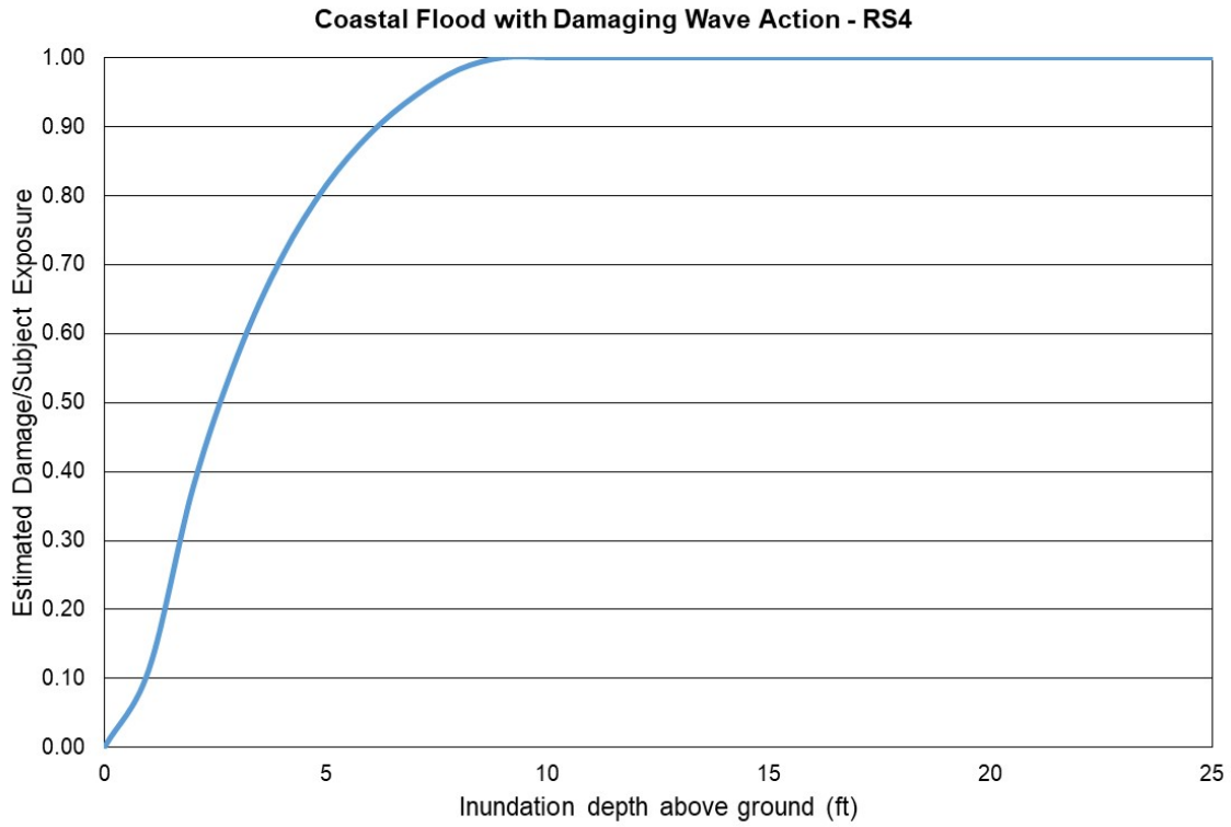
Figure 196. Coastal flood estimated damage vs inundation depth, Reference Building 4.
