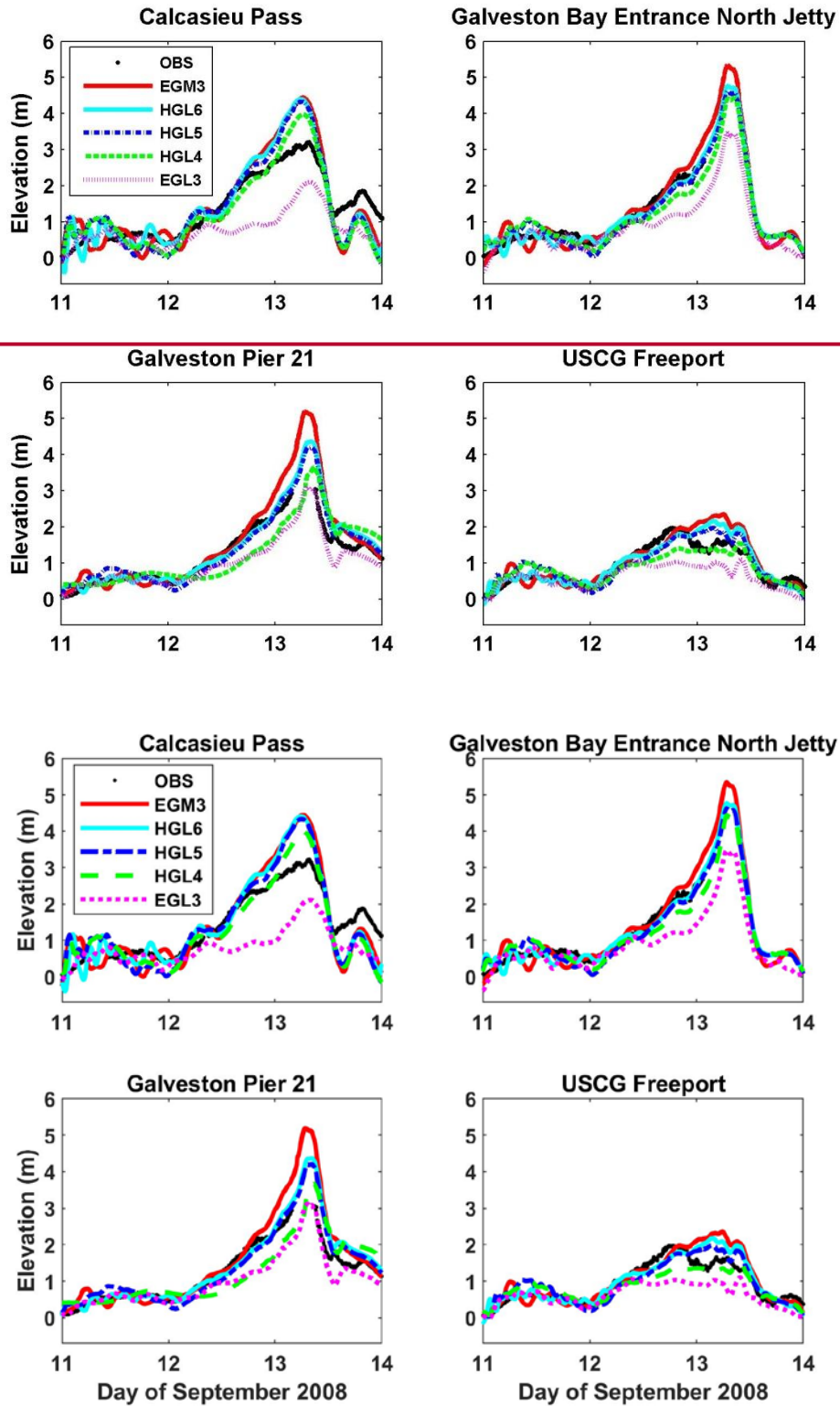
Figure 36. Observed and computed water levels at 4 NOAA tide gauges.
