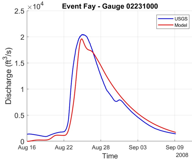
Figure 62. Comparison of the modeled riverine flood flow to recorded flow data for Tropical Storm Fay (2008) from selected USGS gauging station 02231000 located at St. Mary’s River Near Macclenny.
