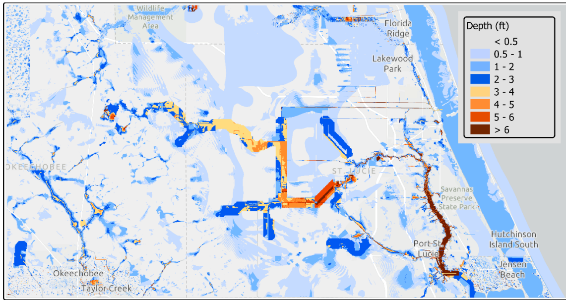
Figure 164. The same as Figure 162 Figure-163 but for region selected in East Florida.
