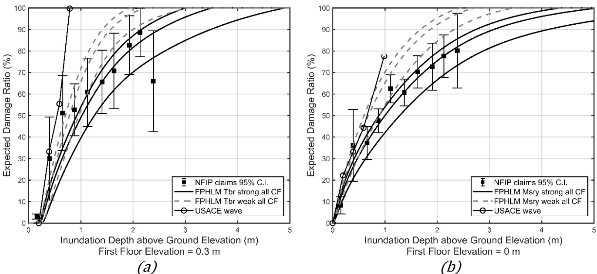
Figure 21. FPFLM Coastal flood (CF) vulnerability, USACE (2015) vulnerability, and Hurricane Ivan 2004 NFIP claims-derived vulnerability relative to the ground elevation a) 1-story slab on-grade timber, 0.3 m FFE; b) 1-story slab on-grade reinforced masonry, 0 m FFE.
