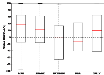
Figure 71. Box Plots of the Relative Difference between Simulated and Observed Streamflow. Note that relative difference is defined as RD\% = 100 * (Q_{sim} - Q_{obs})/Q_{obs} .
