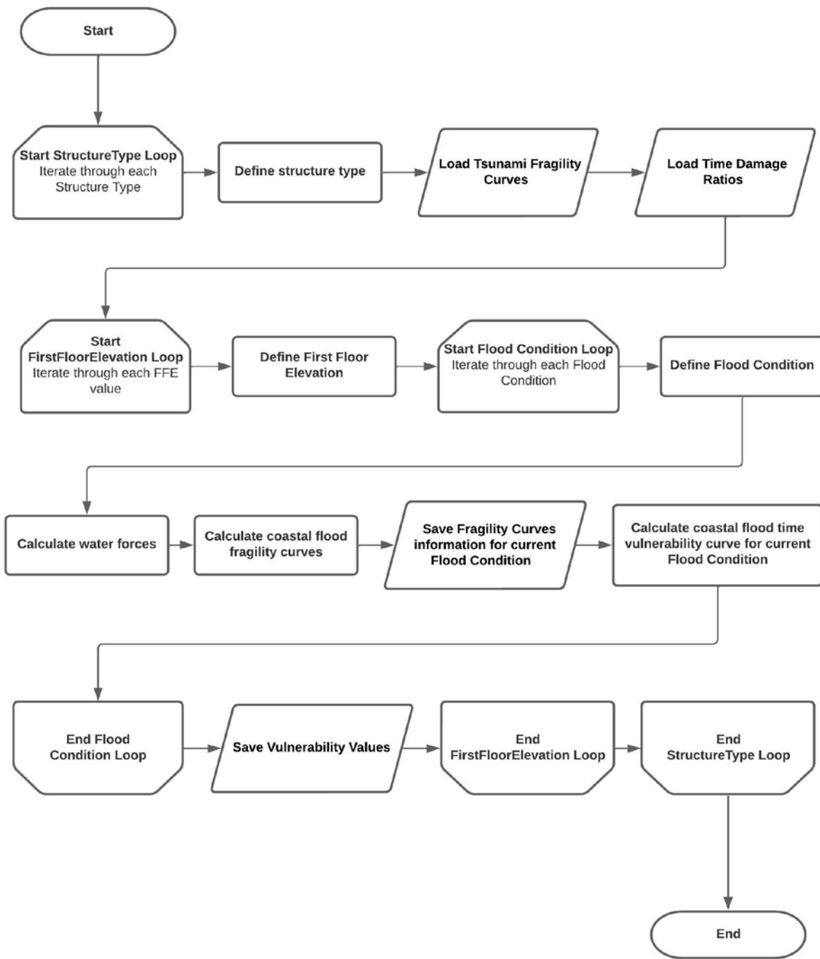
Figure 88. Coastal flood time element vulnerability for buildings.
