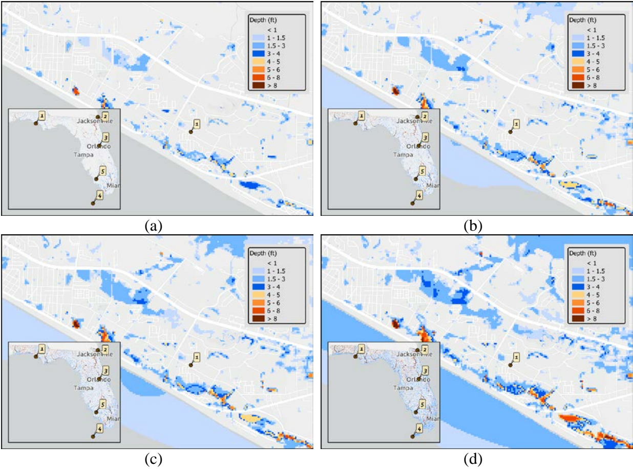
Figure 187. Modeled flood extent and depth for (a) 0.1, (b) 0.02, (c) 0.01, and (d) 0.002 annual exceedance probabilities for the area surrounding the Panama City Beach.
