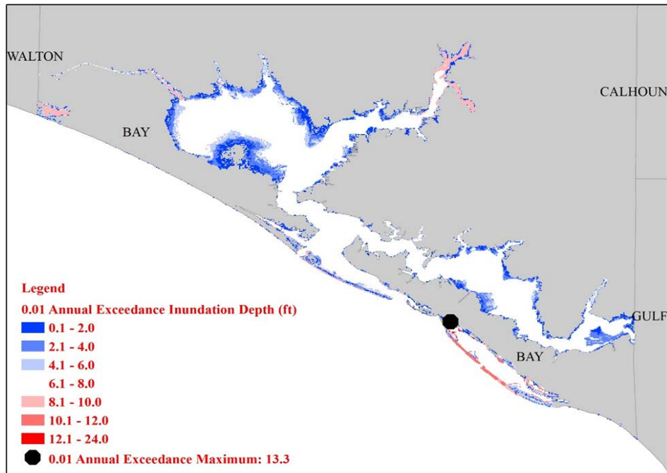
Figure 145. Color-coded contour showing the modeled flood extent and inundation depth corresponding to 0.01 annual exceedance probability at Bay County (Panhandle).
