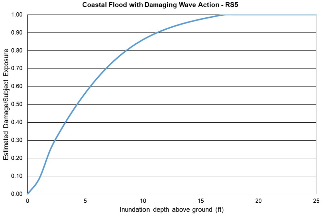
Figure 197. Coastal flood estimated damage vs inundation depth, Reference Building 5.
