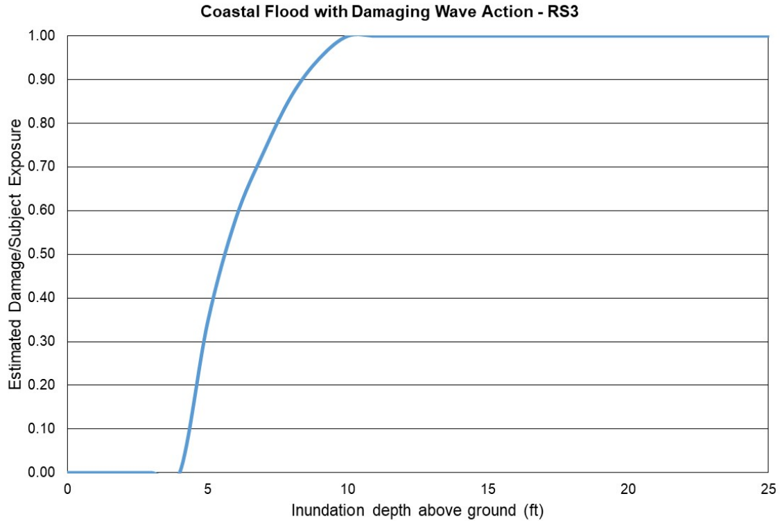
Figure 195. Coastal flood estimated damage vs inundation depth, Reference Building 3.
