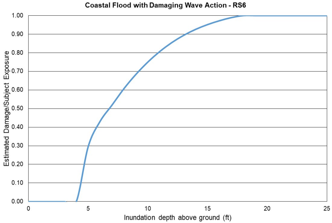
Figure 198. Coastal flood estimated damage vs inundation depth, Reference Building 6.
