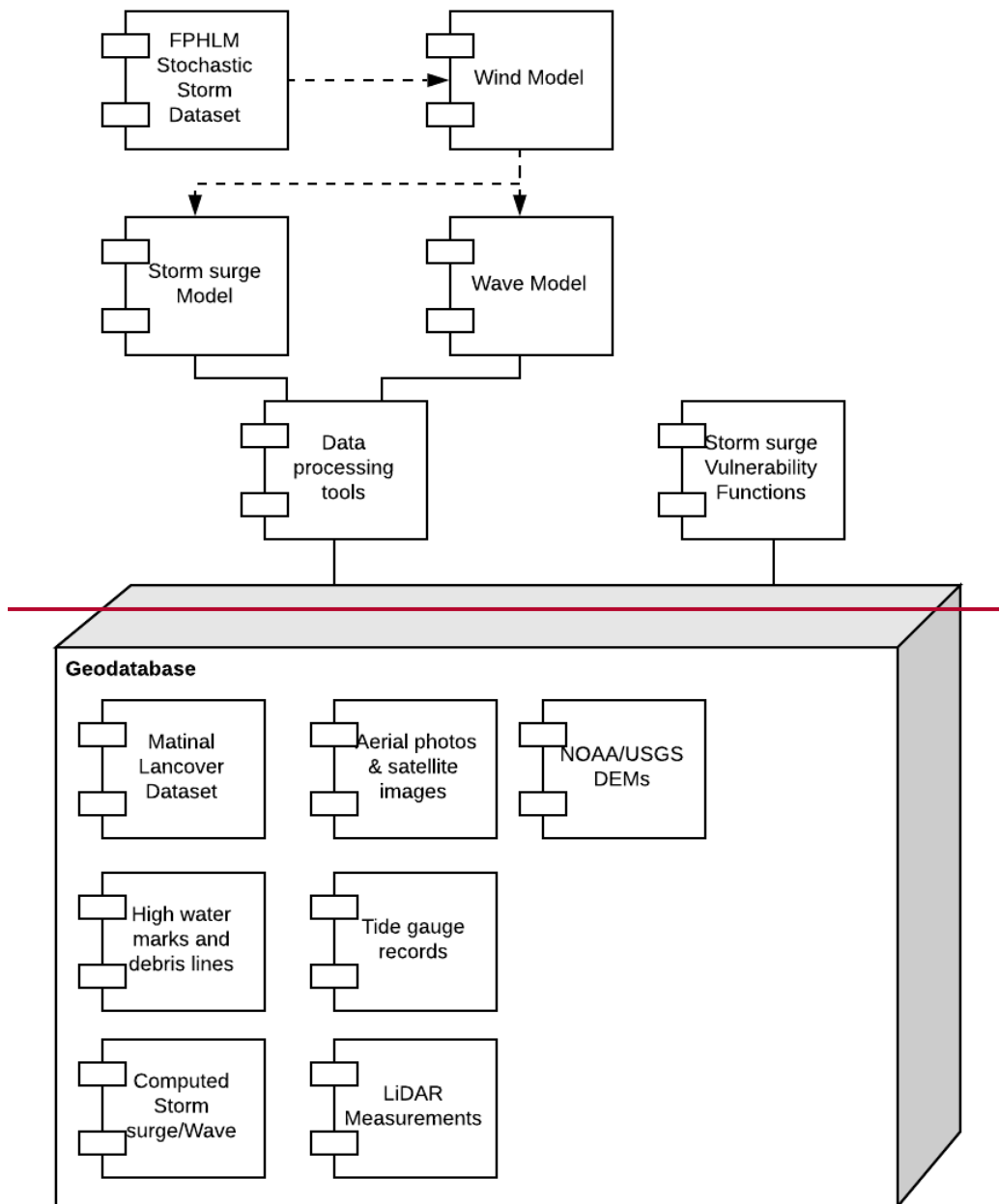
Figure 9. Component diagram of FPFLM with the storm surge.
