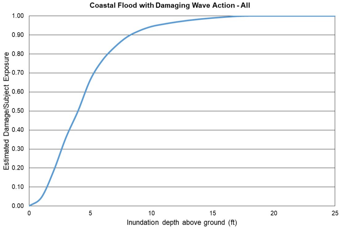
Figure 192. Coastal flood estimated damage vs inundation depth. All reference buildings combined.
