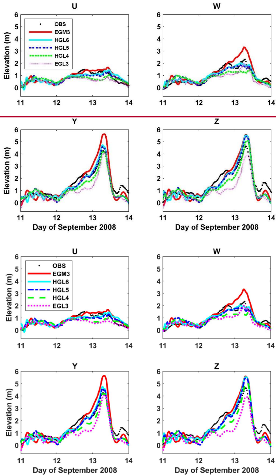
Figure 37. Observed and computed water levels at 4 stations U, W, Y, and Z established by Kennedy Observed and computed water levels at 4 stations established by Kennedy (replace with u,w,y,z).
