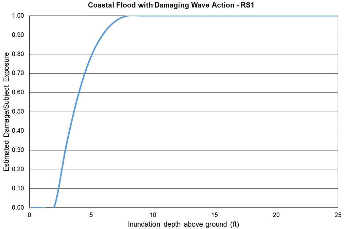
Figure 193. Coastal flood estimated damage vs inundation depth, Reference Building 1.
