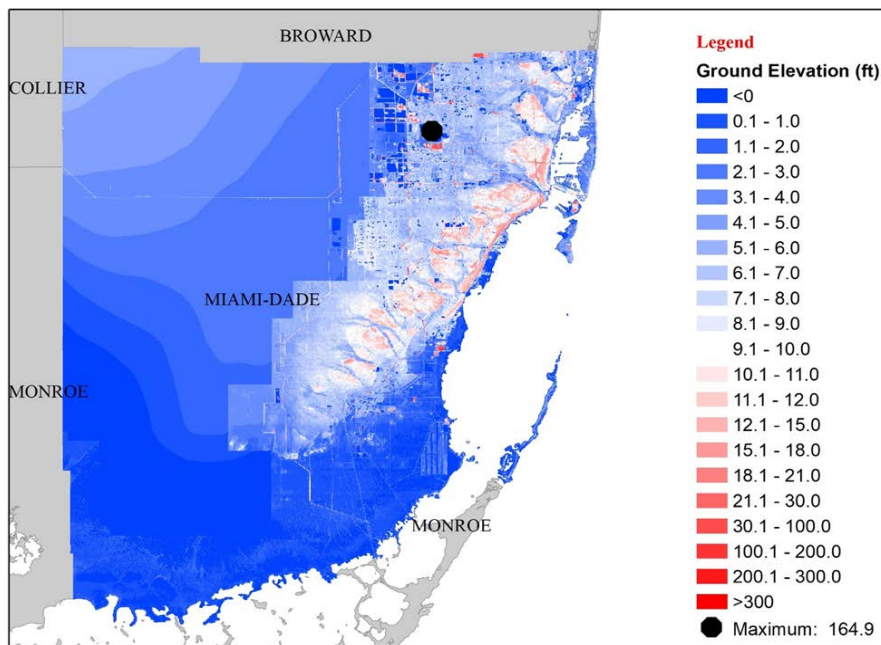
Figure 143. High resolution (100 meters) ground elevation at Miami-Dade County for South East Florida grid.
