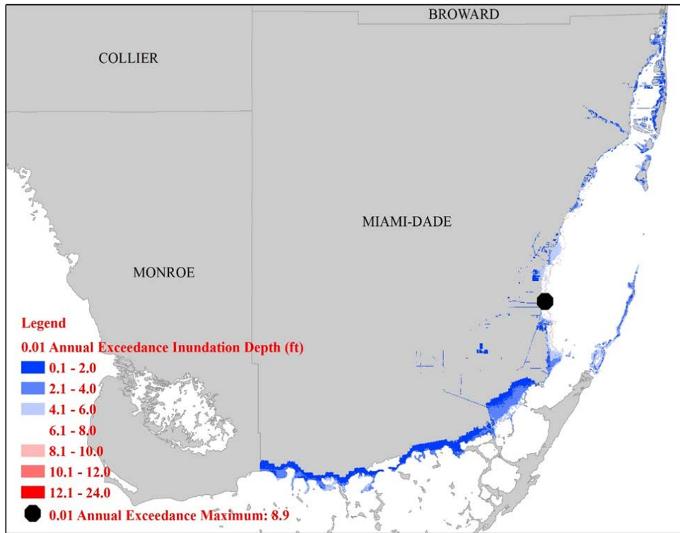
Figure 148. The same as Figure 145 Figure 146 but for Miami-Dade County (South East Florida).
